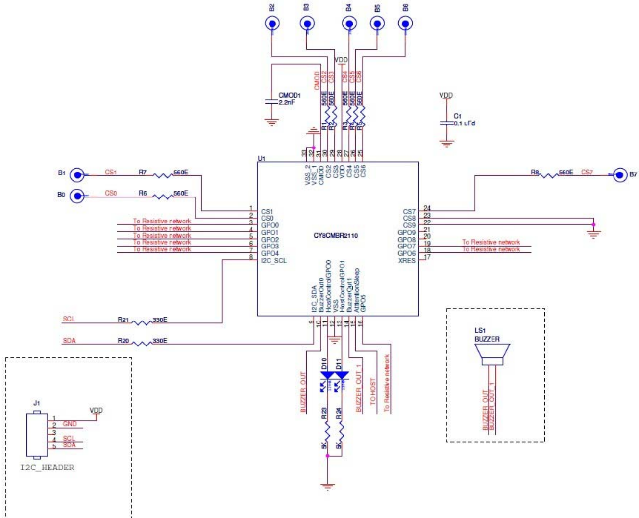
Figure 2. CY8CMBR2110 Schematic 2
