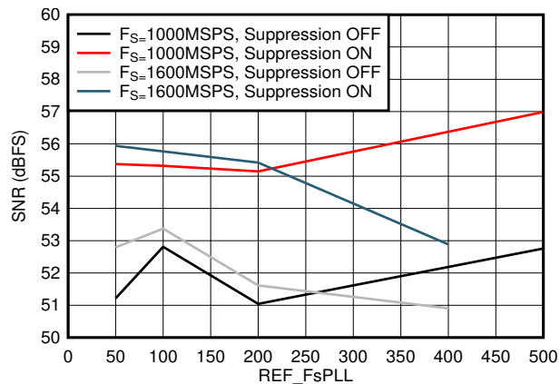
Figure 8-38. SNR vs F_{REF} and Suppression
