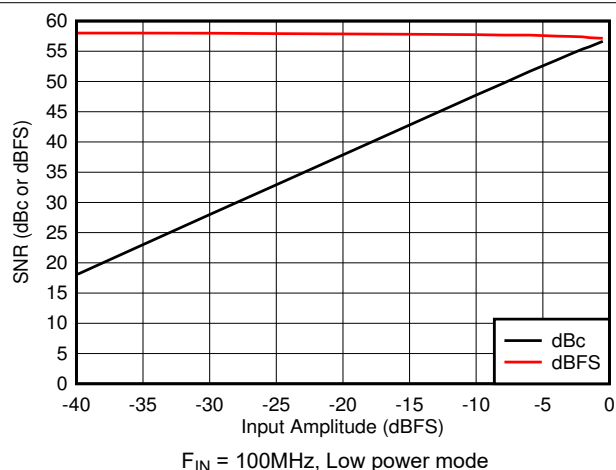
Figure 8-35. SNR vs A_{IN}
