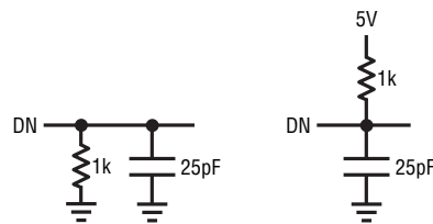
(A) V_{OH} TO Hi-Z
