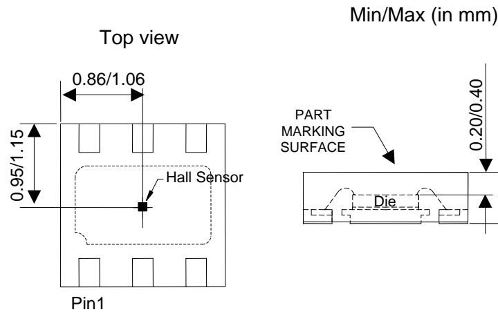
Sensor Location
