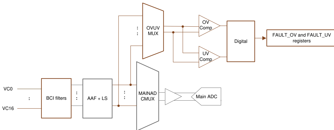
Figure 9-20. OV and UV Protectors
