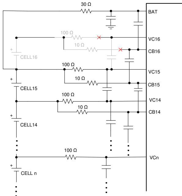
(c) One PCB for all channels applications – For BQ79656: Configured for 15 VC and CB If floating the unused VC and CB pins, capacitors in black corresponding to CB pins need to be populated, but capacitors and resistors in grey corresponding to VC and CB pins need to be unpopulated
