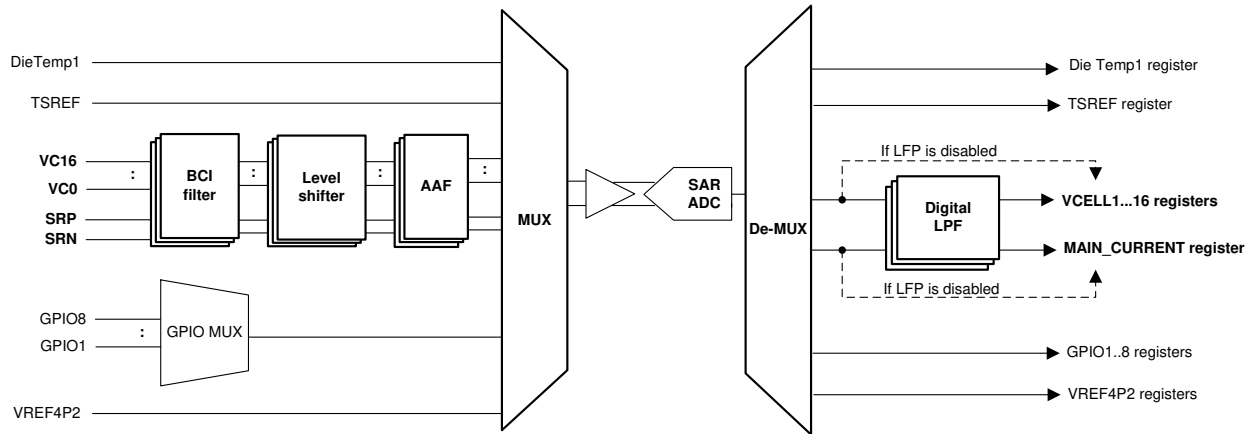
Figure 9-2. Main ADC Measurement Path
