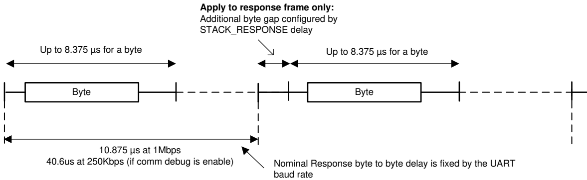
Figure 9-35. Daisy Chain Byte Transfer
