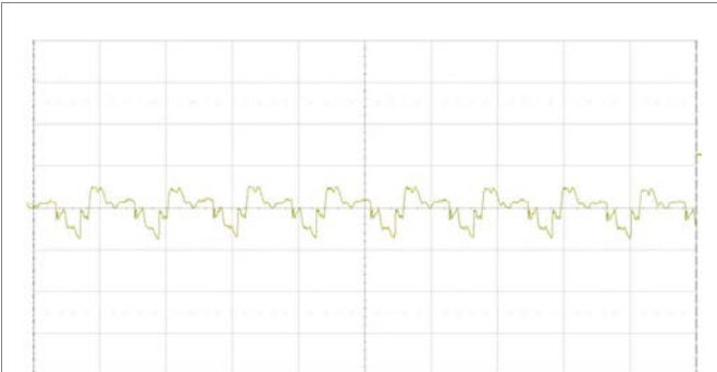
Output voltage ripple at: T_{P1} = +25^{\circ}\text{C} , V_I = 48\text{ V} , I_O = 10\text{ A} resistive load. Trace: output voltage (20 mV/div.). Time scale: (2 μs/div.). 20 MHz bandwidth.
