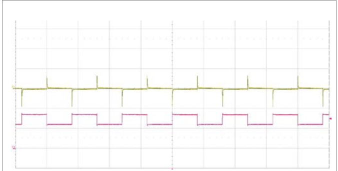
Output voltage response to load current step-change (2.1-3.15-2.1 A) at: T_{P1} = +25^{\circ}\text{C} , V_I = 48\text{ V} . Top trace: output voltage (500 mV/div.). Bottom trace: load current (2 A/div.). Time scale: (10 ms/div.).
