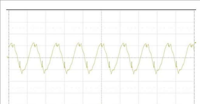
Output voltage ripple at: T_{P1} = +25^{\circ}\text{C} , V_I = 48\text{ V} , I_o = 4.2\text{ A} resistive load. Trace: output voltage (20 mV/div.). Time scale: (2 μs/div.). 20 MHz bandwidth.
