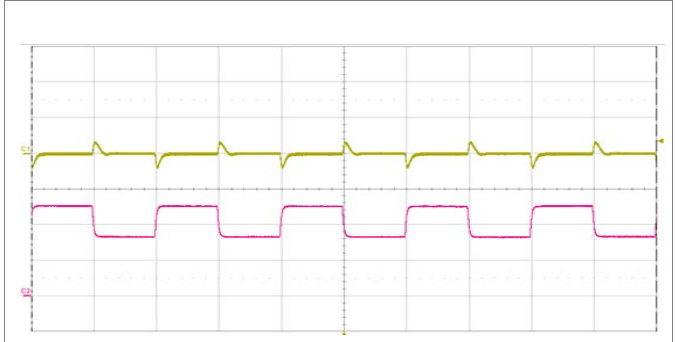
Output voltage response to load current step- change (1.7-2.55-1.7 A) at: T_{P1} = +25^{\circ}\text{C} , V_I = 48\text{ V} . Top trace: output voltage (500 mV/div.). Bottom trace: load current (1 A/div.). Time scale: (2 ms/div.).
