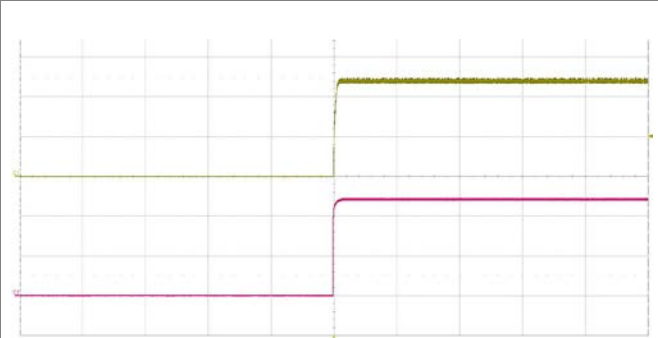
Start-up enabled by connecting V_I at: T_{P1} = +25^{\circ}\text{C} , V_I = 48\text{ V} , I_o = 4.2\text{ A} resistive load. Top trace: output voltage (5 V/div.). Bottom trace: input voltage (20 V/div.). Time scale: (200 ms/div.).
