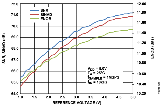
Figure 19. SNR, SINAD, and ENOB vs. Reference Voltage
