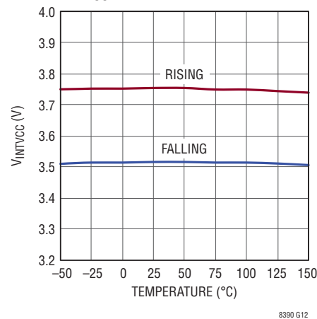
V_{INTVCC} UVLO Threshold
