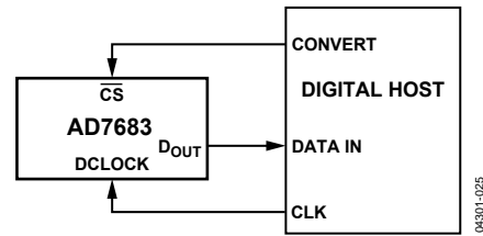
Figure 26. Connection Diagram
