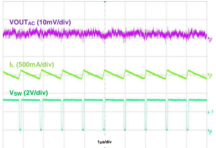
Figure 50. Output Voltage Ripple, V_{IN} = 3\text{V} , V_{OUT} = 3.3\text{V} , I_{OUT} = 50\text{mA}
