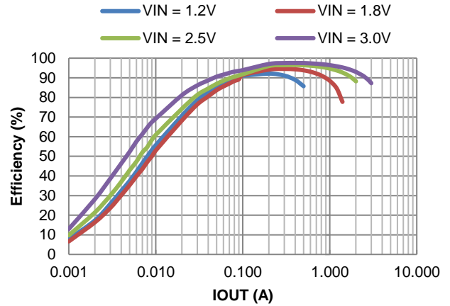
Figure 42. Efficiency vs. Output Current, V_{OUT} = 3.3\text{V}
