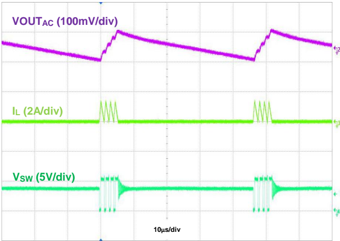
Figure 20. Output Voltage Ripple, V_{OUT} = 5.2\text{V} , I_{OUT} = 50\text{mA}
