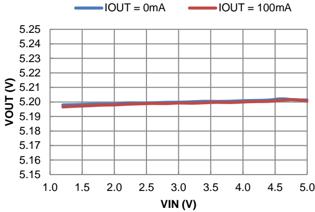
Figure 43. Line Regulation
