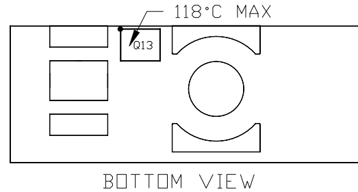
Figure 20. Temperature reference points on bottom side
