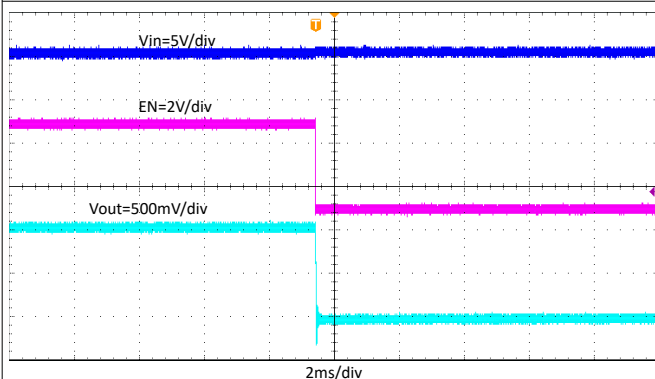
Figure 8-16. Shutdown Through EN, I_{OUT} = 5\text{ A}
