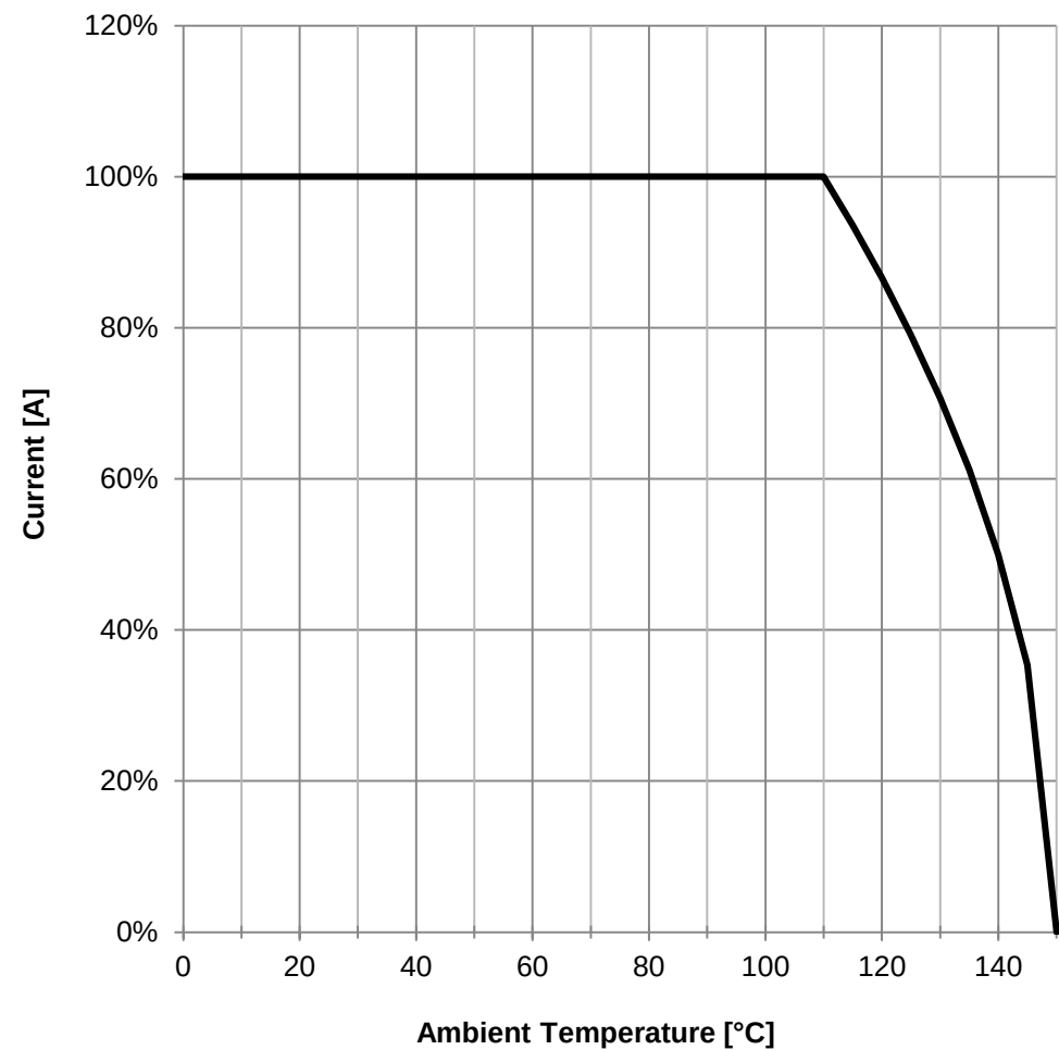
Derating Curve:
