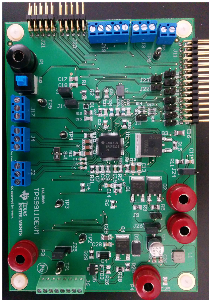
Figure 1. TPS99110EVM Board
