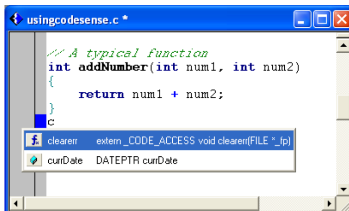
Figure 4-11. Code Sense
