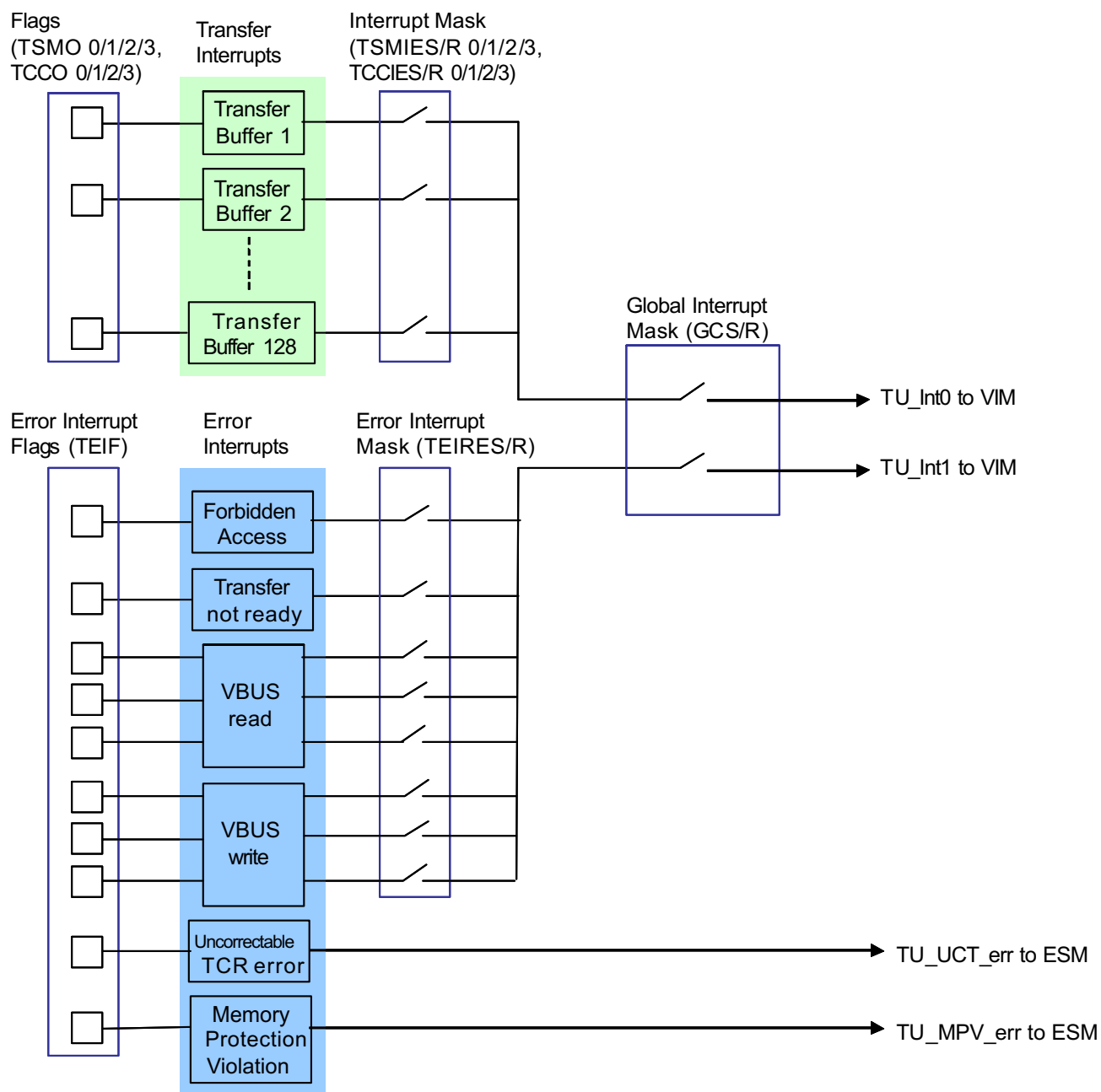
Figure 23-28. Transfer Unit (TU) Interrupt Structure
