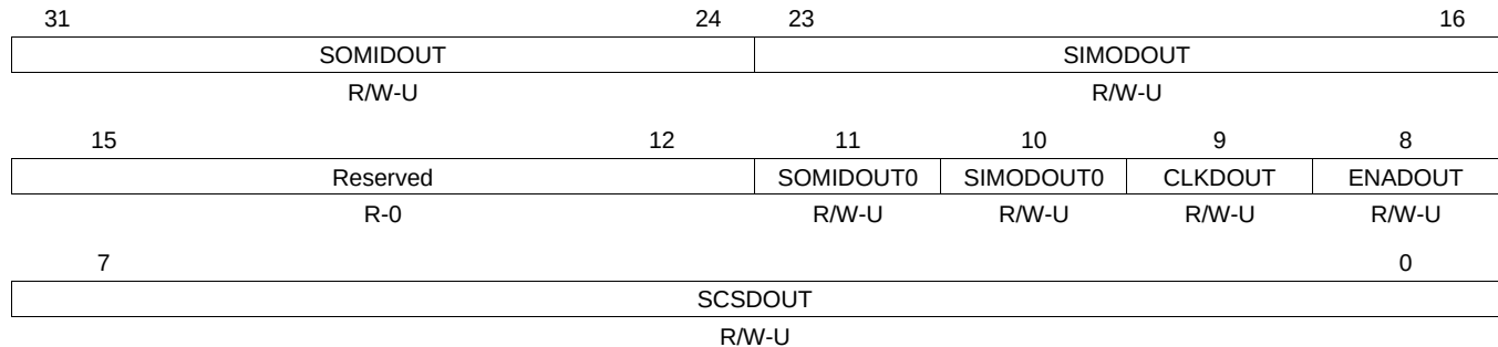
Figure 25-34. SPI Pin Control Register 3 (SPIPC3) [offset = 20h]
