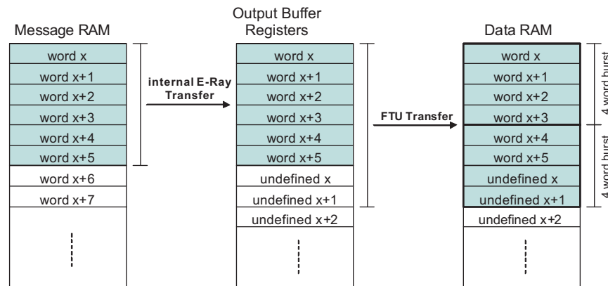
Figure 23-7. Example: FTU Read Transfer of 6 Words
