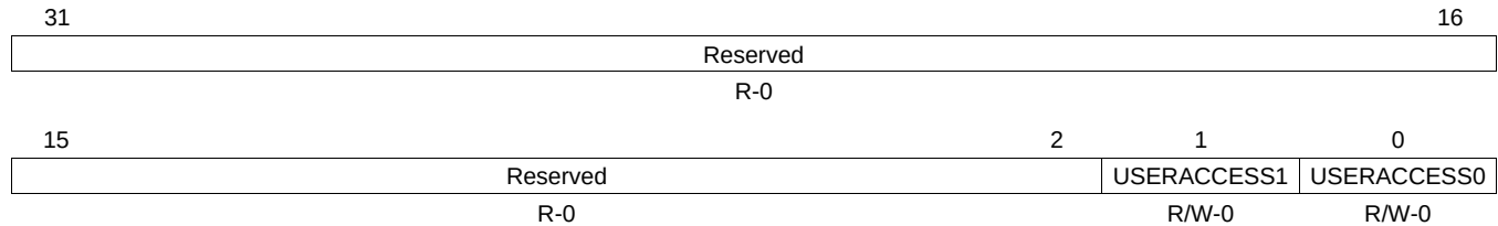
Figure 29-36. MDIO User Command Complete Interrupt Mask Set Register (USERINTMASKSET)
