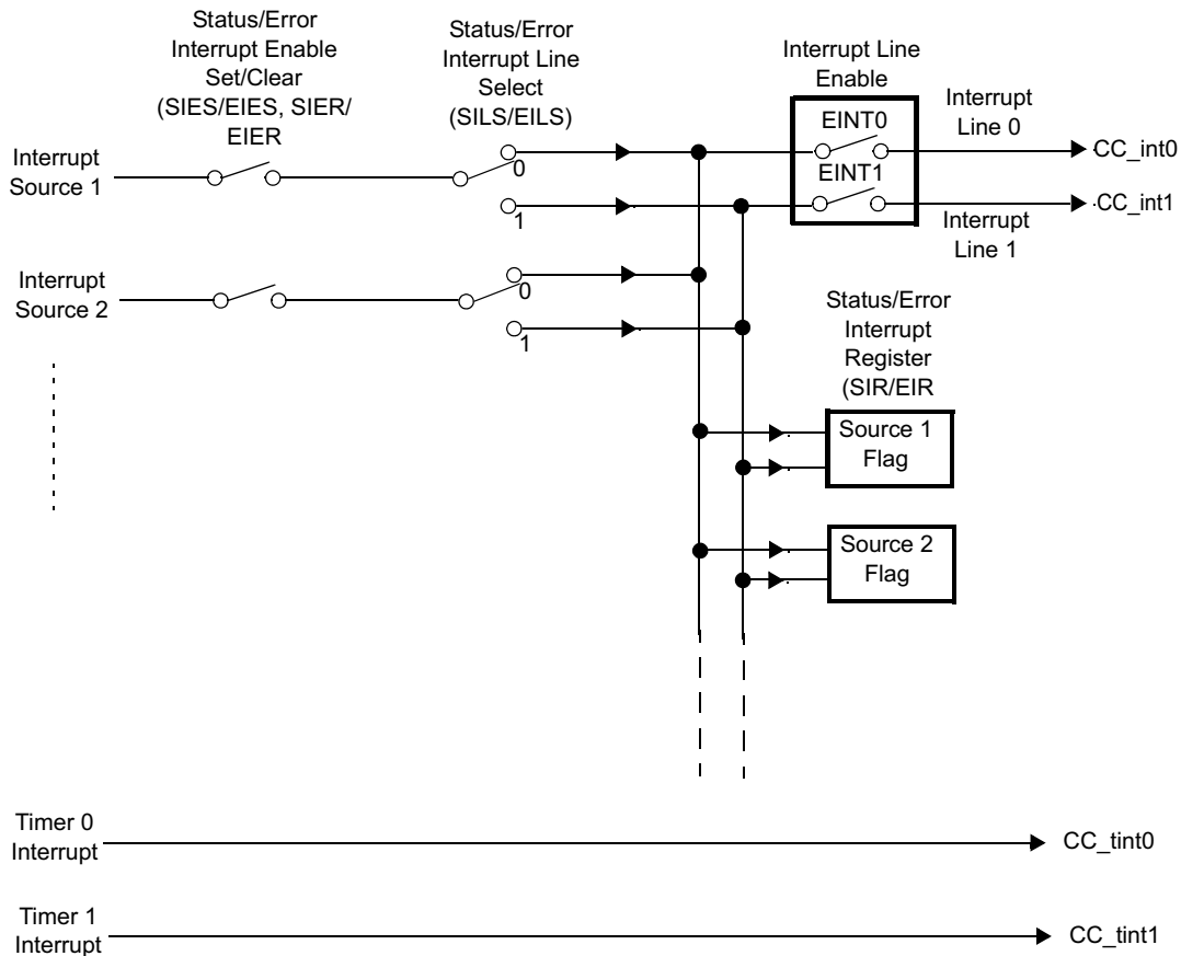
Figure 23-29. Communication Controller (CC) Interrupt Structure
