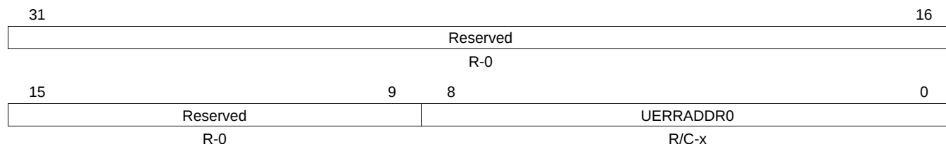
Figure 25-71. TXRAM Uncorrectable Parity Error Address Register (UERRADDR0) [offset = 12Ch]
