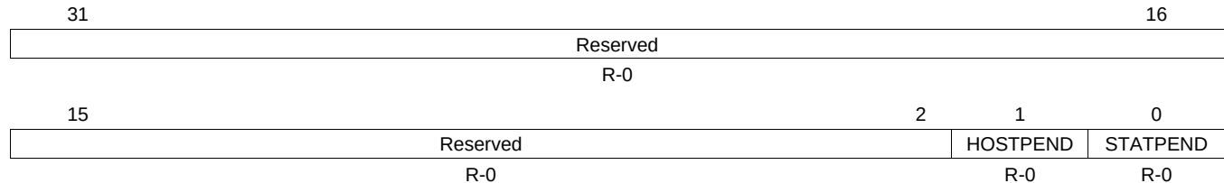
Figure 29-58. MAC Interrupt Status (Unmasked) Register (MACINTSTATRAW)
