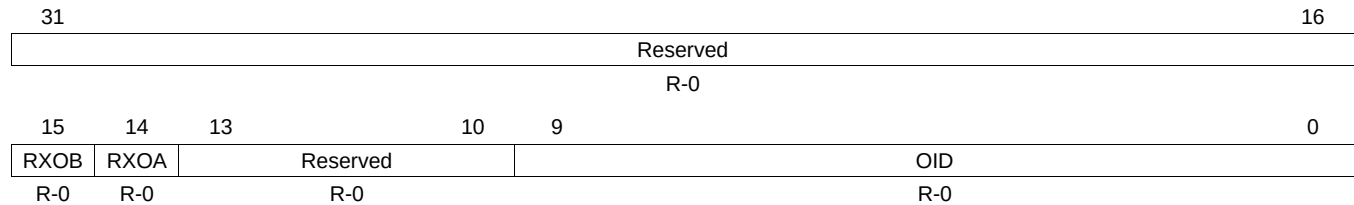
Figure 23-149. Odd Sync ID Registers (OSIDn) [offset_CC = 170h-1A8h]
