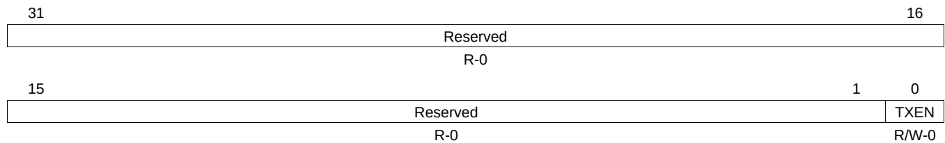
Figure 29-43. Transmit Control Register (TXCONTROL)
