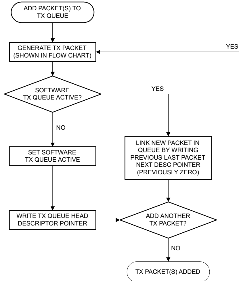
Figure 29-7. Transmit Packet Add Flow Chart
