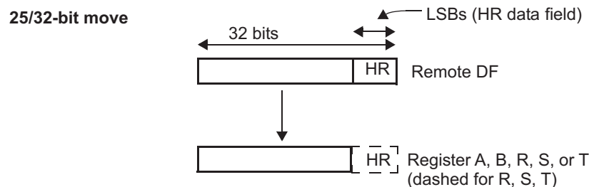
Figure 20-159. MOV32 Move Operation for REMTOREG (Case 11)
