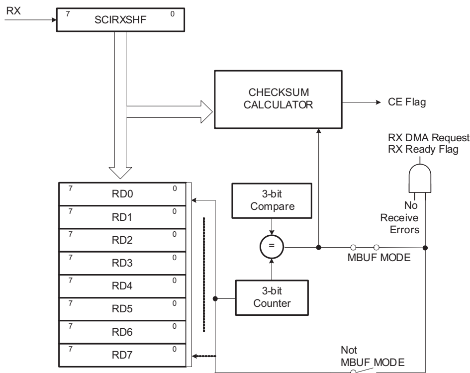
Figure 26-8. Receive Buffers
