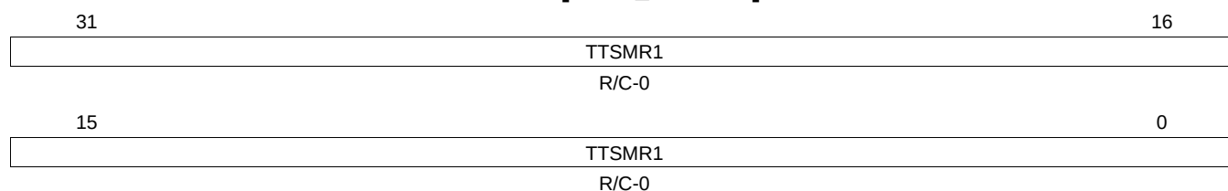
Figure 23-56. Trigger Transfer to System Memory Reset 1 (TTSMR1) [offset_TU = 84h]
