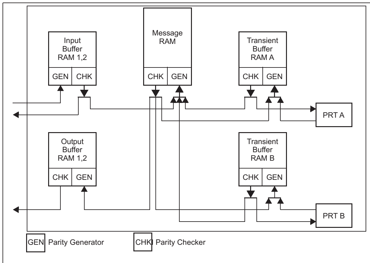
Figure 23-27. Parity Generation and Check
