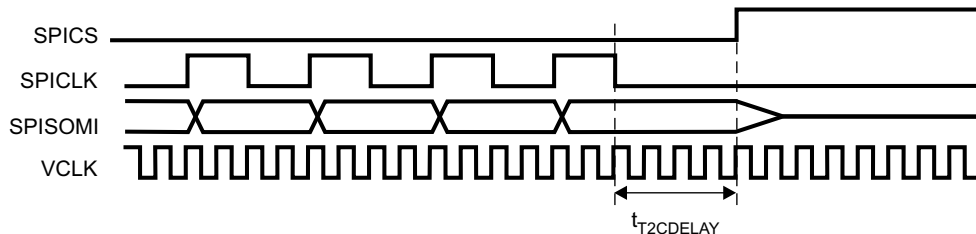
Figure 25-46. Example: t_{T2CDELAY} = 4 VCLK Cycles
