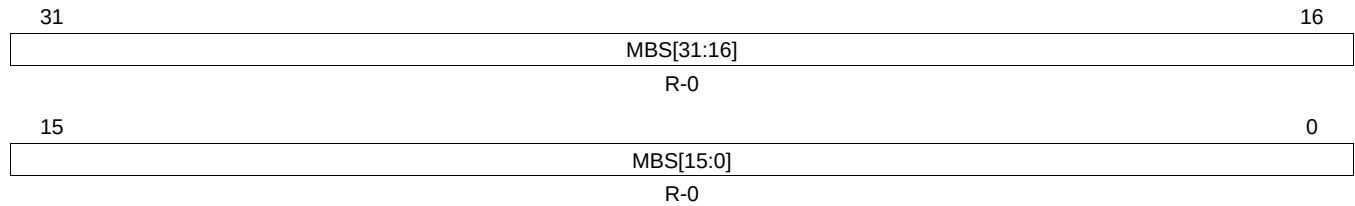
Figure 23-167. Message Buffer Status Changed Register 1 (MBSC1) [offset_CC = 340h]
