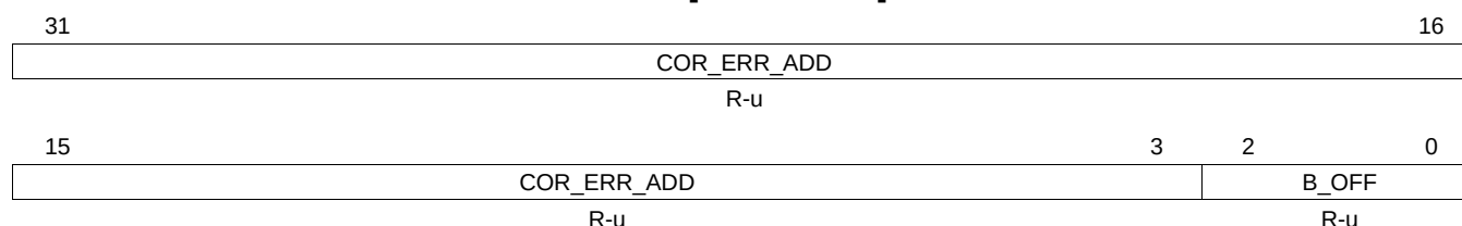
Figure 5-44. EEPROM Emulation Correctable Error Address Register (EE_COR_ERR_ADD) [offset = 314h]
