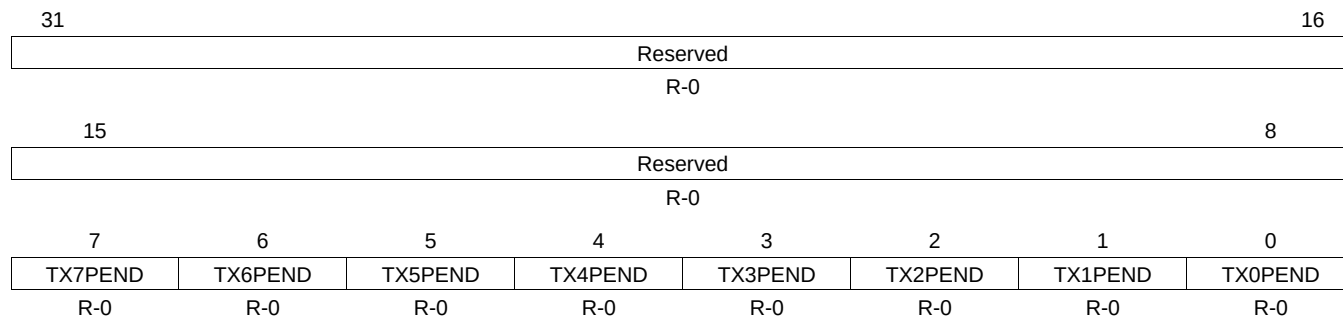
Figure 29-49. Transmit Interrupt Status (Masked) Register (TXINTSTATMASKED)
