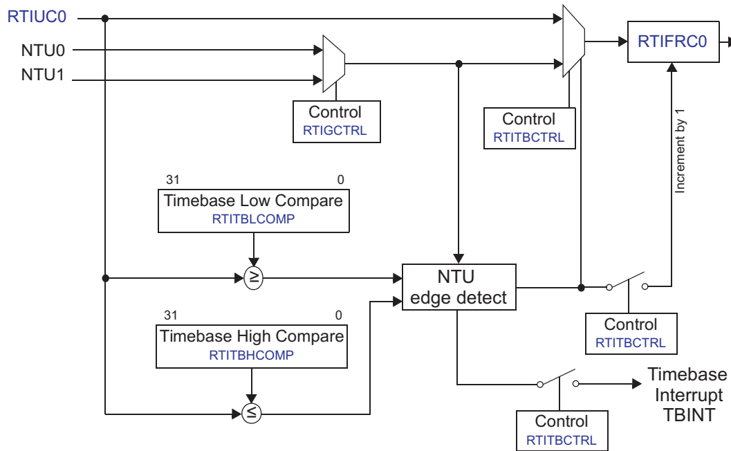
Figure 13-4. Timebase Control
