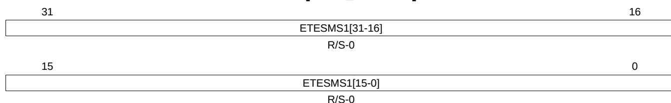
Figure 23-71. Enable Transfer on Event to System Memory Set 1 (ETESMS1) [offset_TU = C0h]
