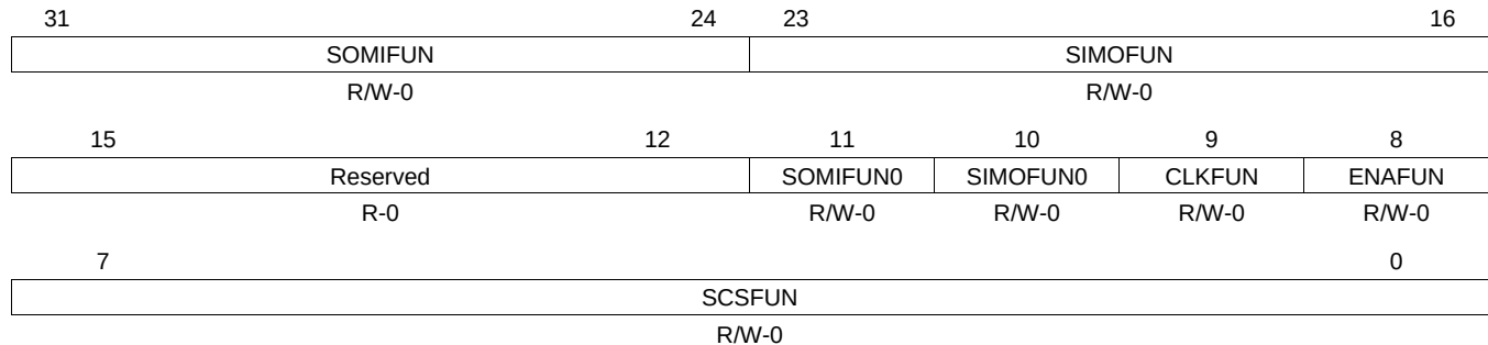
Figure 25-31. SPI Pin Control Register 0 (SPIPC0) [offset = 14h]
