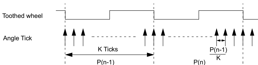
Figure 20-37. Angle Tick Generation Principle
