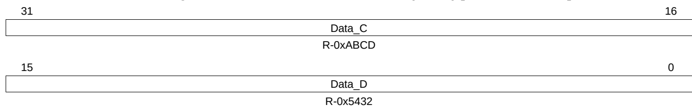
Figure 23-31. Global Static Number 1 (GSN1) [offset_TU = 04h]
