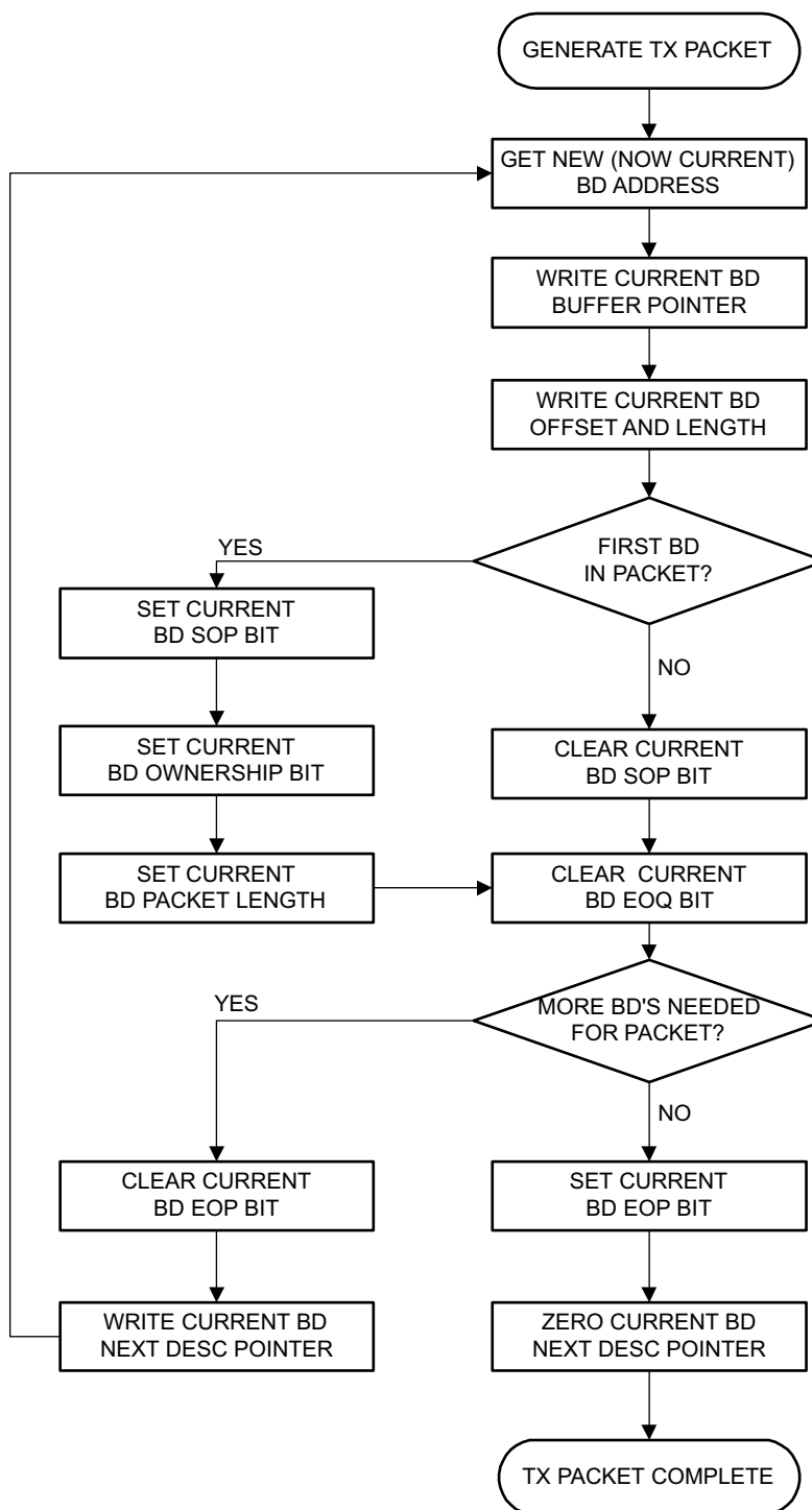
Figure 29-8. Generate Transmit Packet Flow Chart
