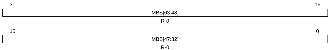
Figure 23-168. Message Buffer Status Changed Register 2 (MBSC2) [offset_CC = 344h]
