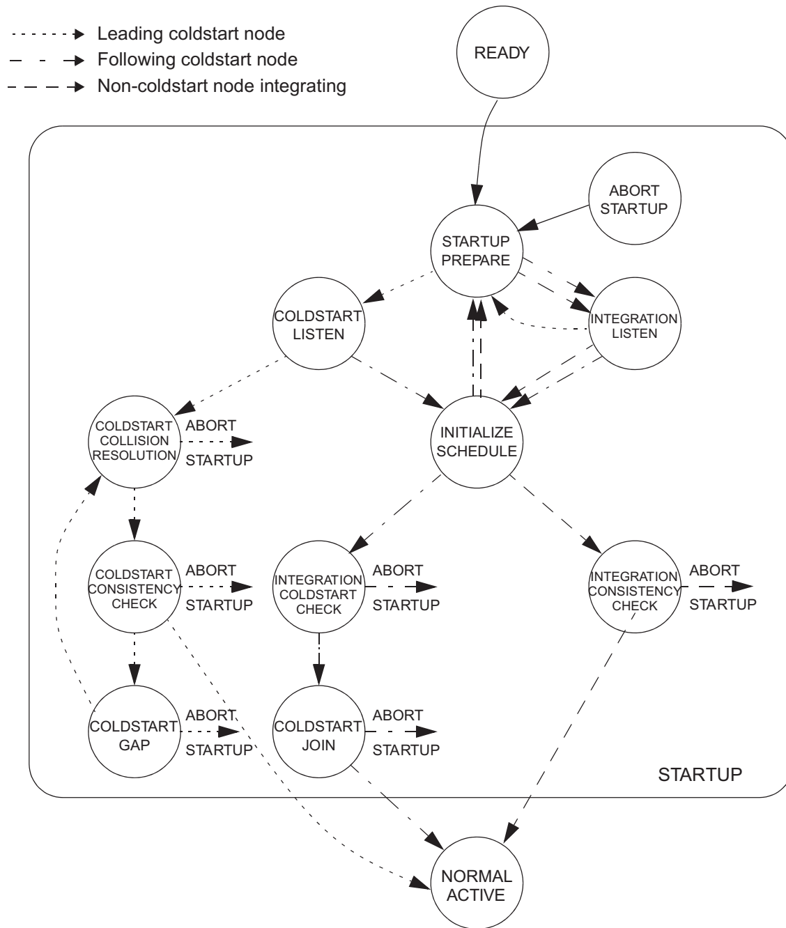
Figure 23-15. State Diagram Time-Triggered Startup
