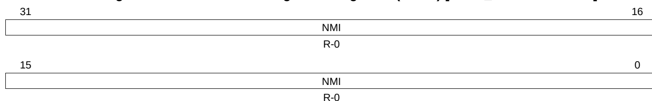
Figure 23-150. Network Management Registers (NMVn) [offset_CC = 1B0h-1B8h]
