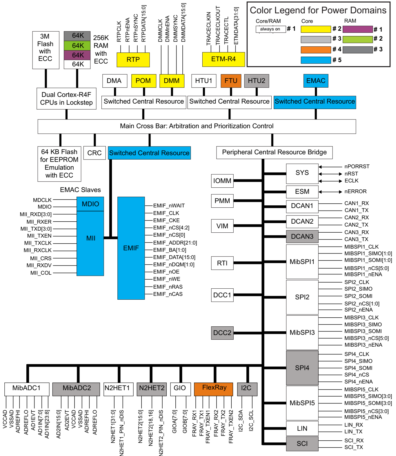
Figure 1-1. Block Diagram
