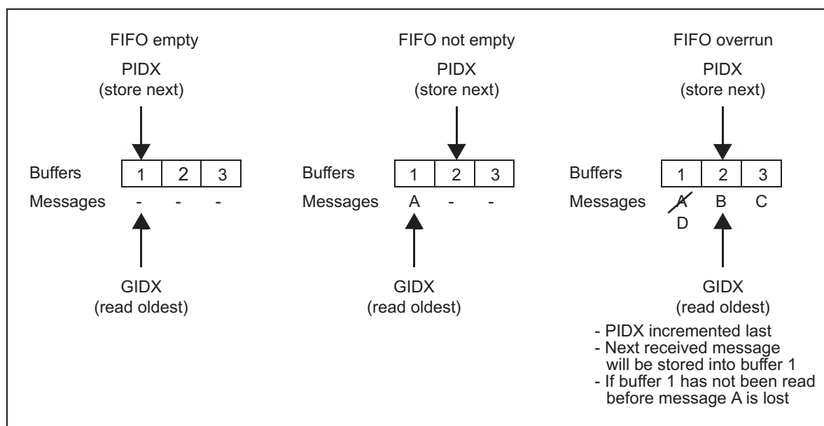
Figure 23-16. FIFO Status: Empty, Not Empty, and Overrun
