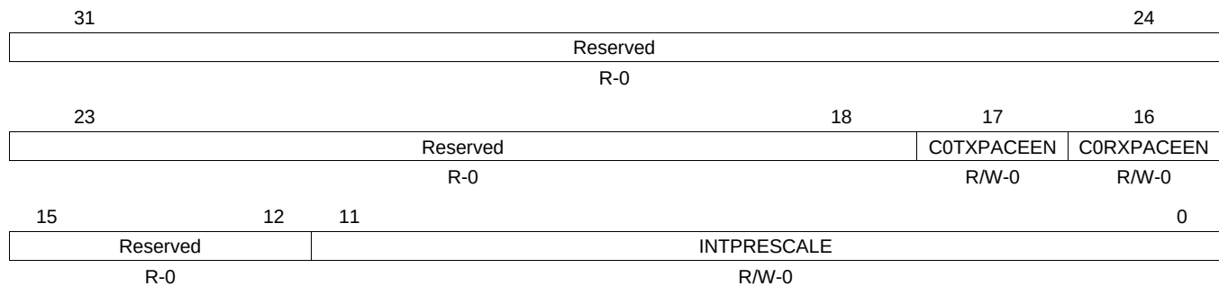
Figure 29-17. EMAC Control Module Interrupt Control Register (INTCONTROL)
