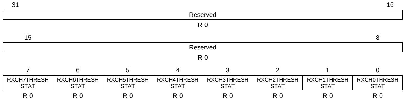
Figure 29-22. EMAC Control Module Receive Threshold Interrupt Status Register (C0RXTHRESHSTAT)
