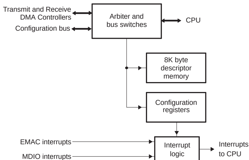
Figure 29-12. EMAC Control Module Block Diagram
