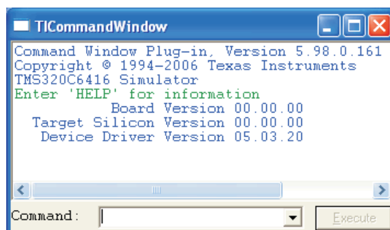
Figure 5-21. Command Window
