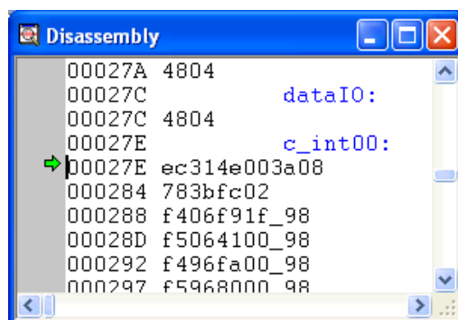
Figure 5-18. Disassembly Window
