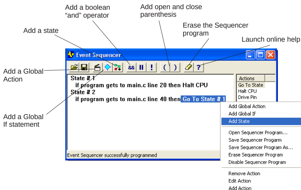
Figure 5-26. Event Sequencer
