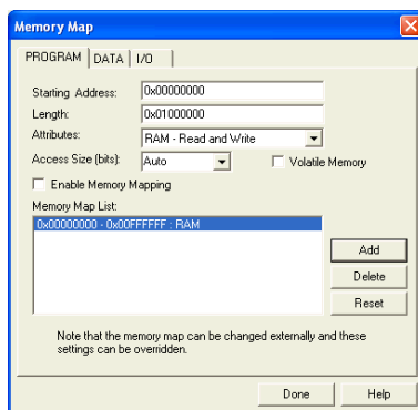
Figure 5-2. Memory Map
