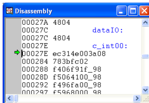
Figure 5-18. Disassembly Window
