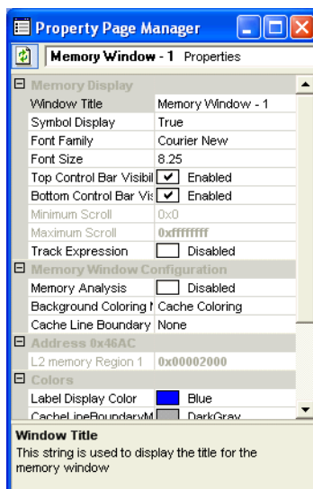
Figure 5-11. Property Window
