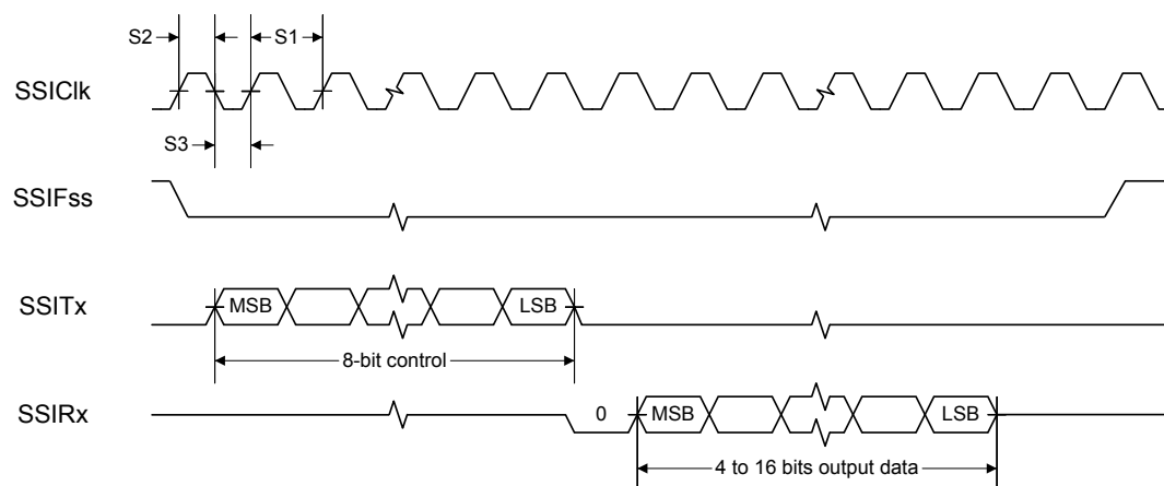
Figure 19-15. SSI Timing for MICROWIRE Frame Format (FRF=10), Single Transfer
