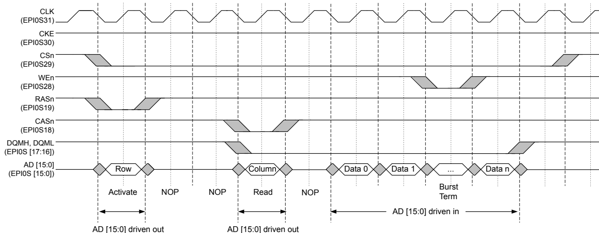
Figure 10-2. SDRAM Non-Blocking Read Cycle
