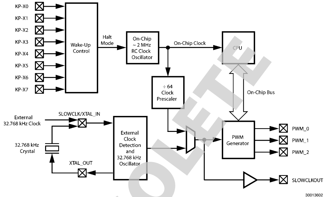
FIGURE 2. Clock Architecture
