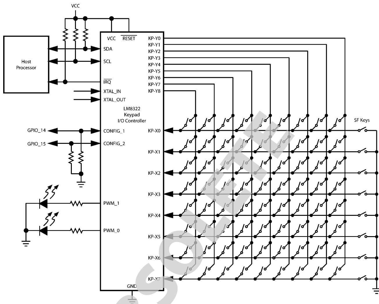
FIGURE 1. Typical Application
