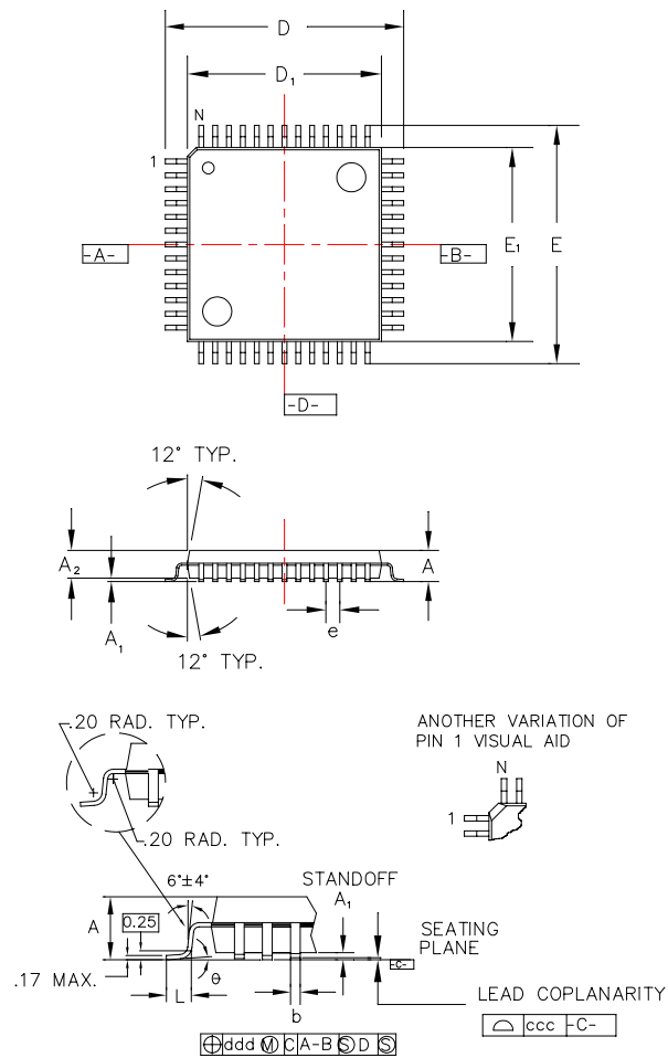
Figure C-1. Stellaris LM3S8G62 100-Pin LQFP Package Dimensions
