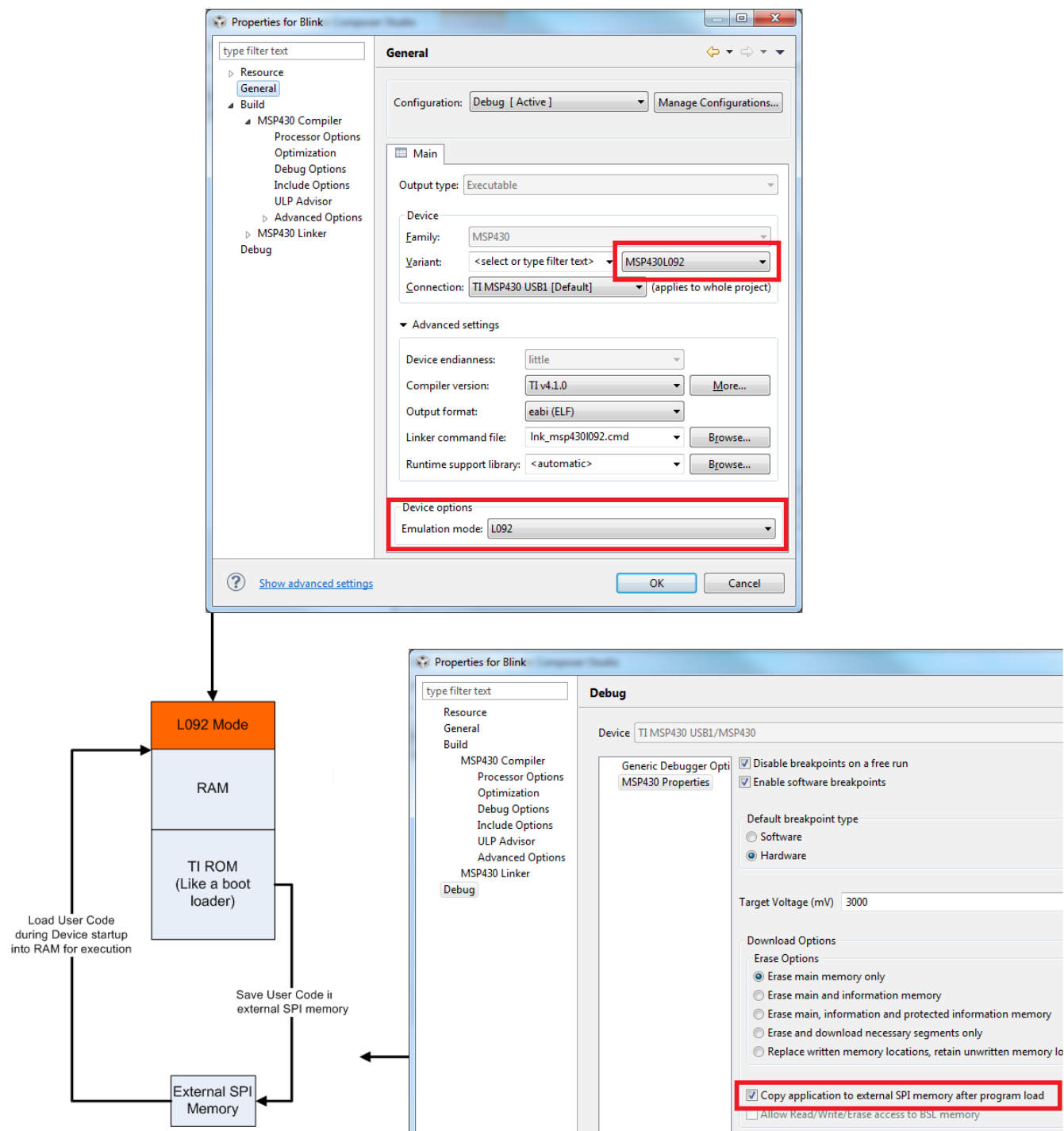
Figure 11-1. MSP430L092 Modes
