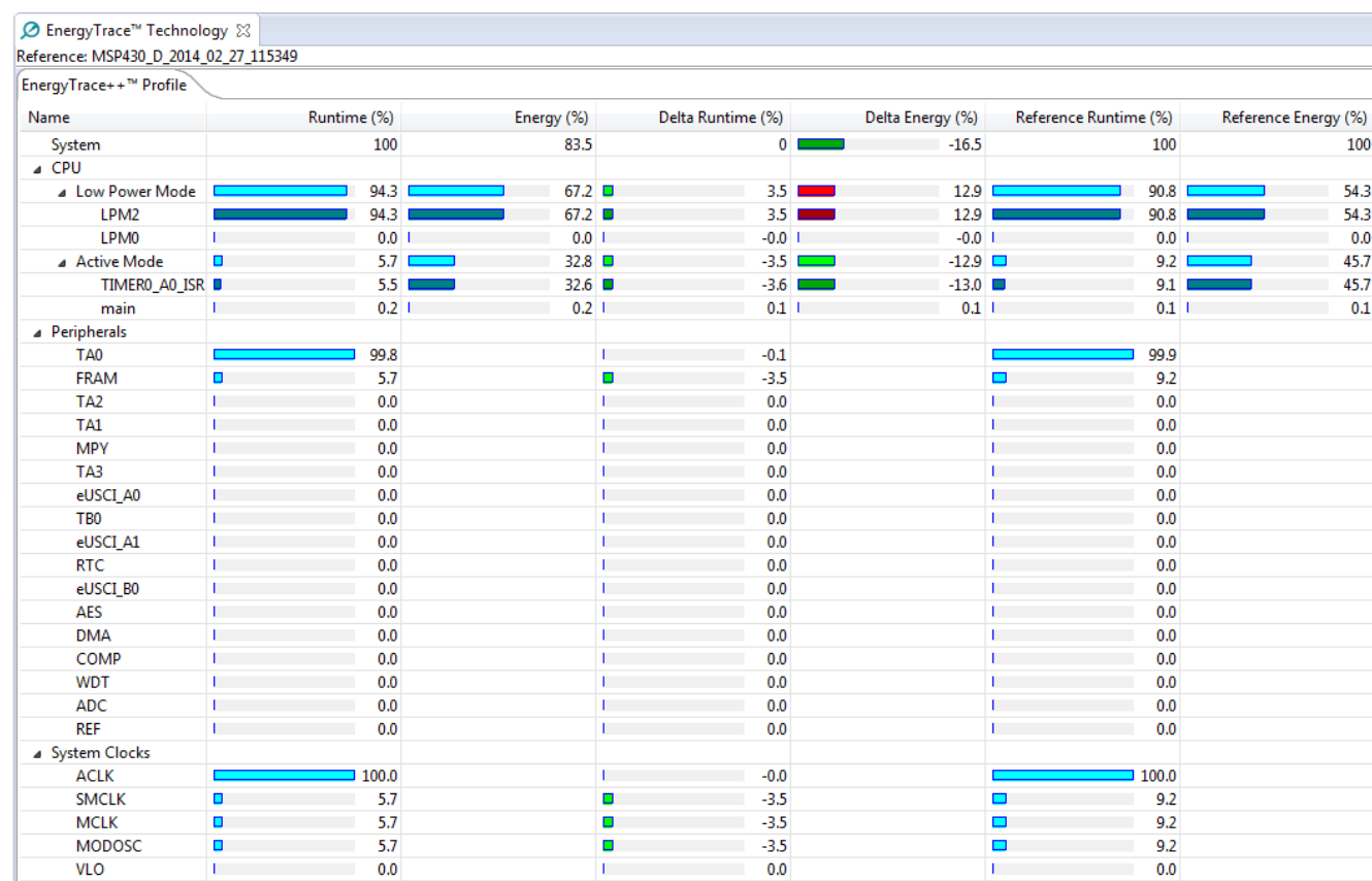
Figure 4-21. Comparing Profiles in EnergyTrace++ Mode
