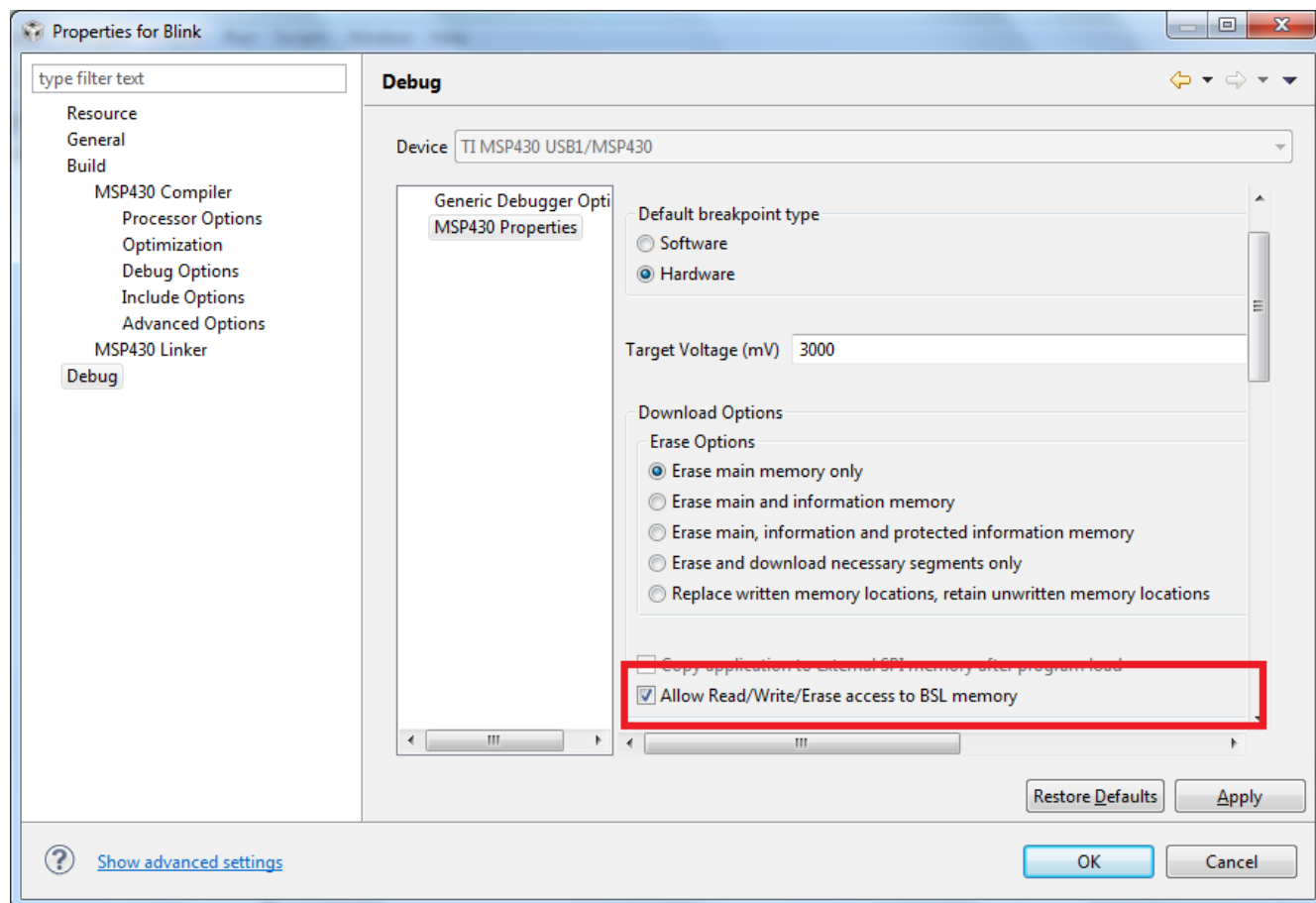
Figure 11-4. Allow Access to BSL
