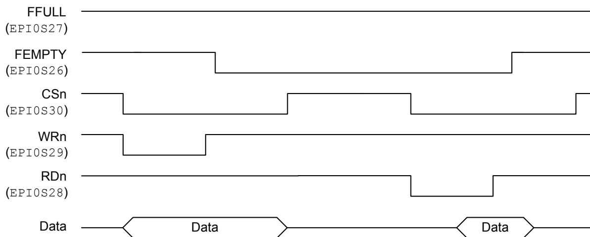
Figure 9-11. Two-Entry FIFO
