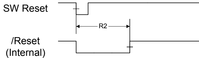
Figure 26-11. Software Reset Timing
