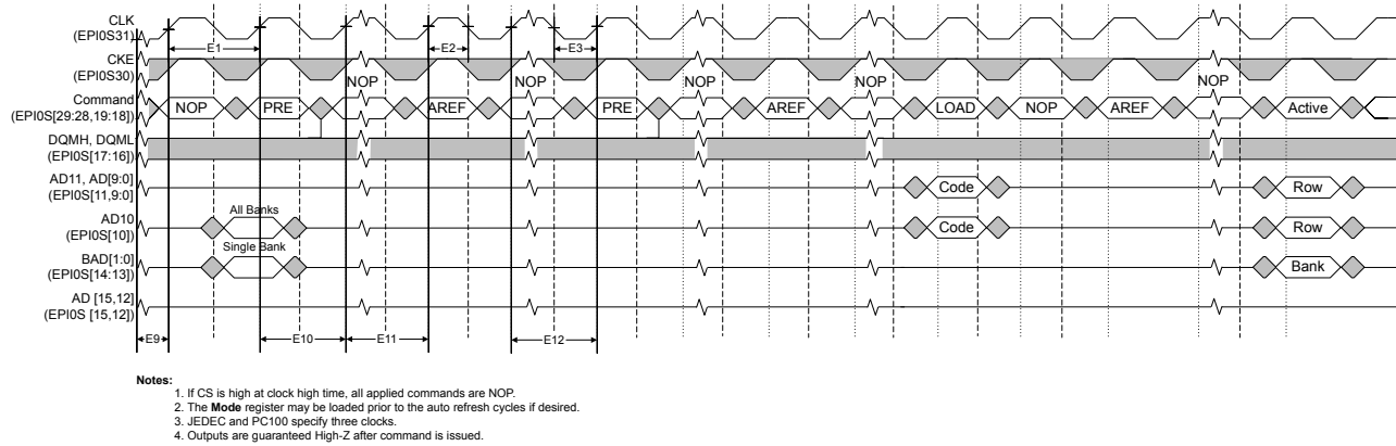
Figure 26-14. SDRAM Initialization and Load Mode Register Timing
