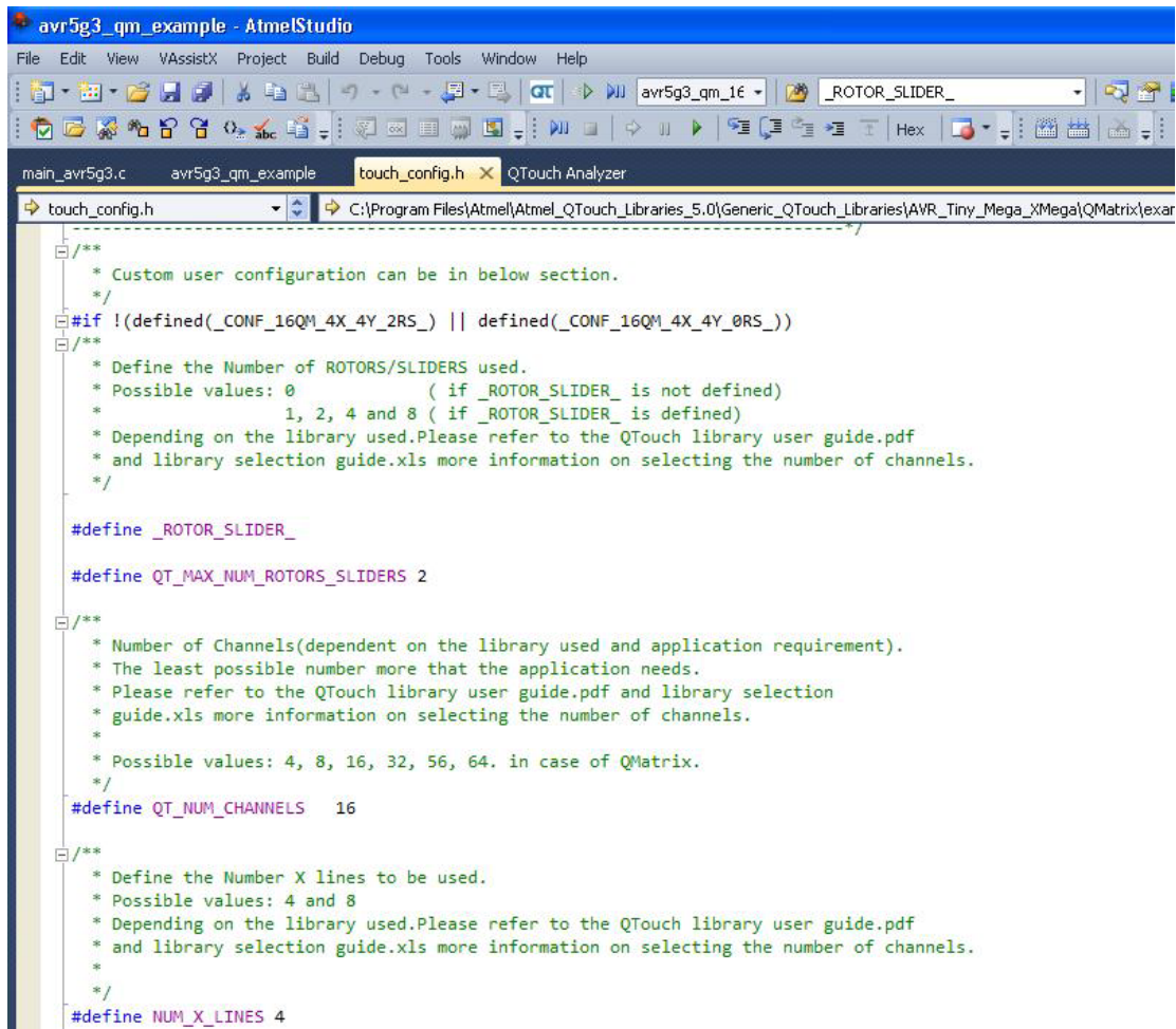
Figure 5-18 : Specifying QMatrix acquisition library parameters in touch_config.h for QMatrix projects
