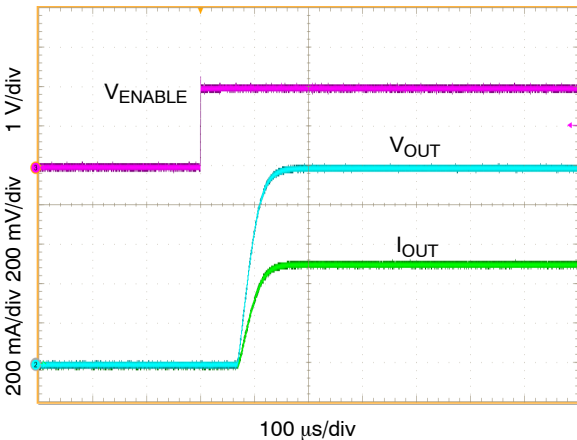
Figure 15. Enable Turn-on Response, Output Resistive Load 500\text{ mA} , C_{OUT} = 10\ \mu\text{F}
