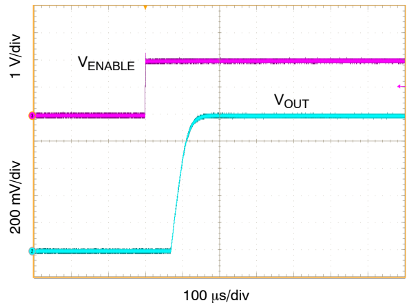
Figure 16. Enable Turn-on Response, I_{OUT} = 0\text{ mA} , C_{OUT} = 2.2\ \mu\text{F}
