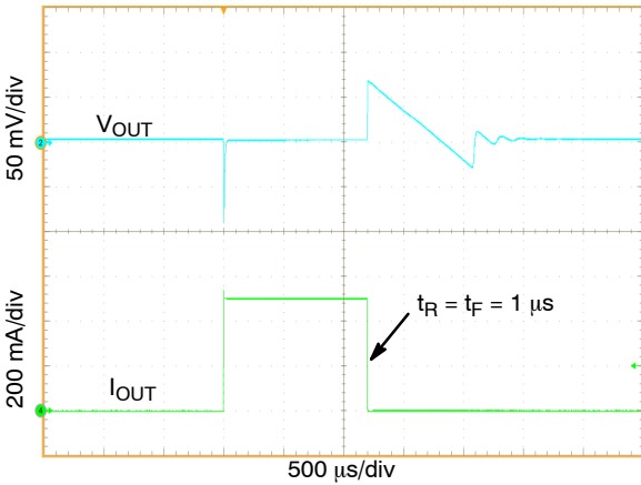
Figure 13. Load Transient Response, I_{OUT} = 1\text{ mA} to 500\text{ mA} , C_{OUT} = 10\ \mu\text{F}
