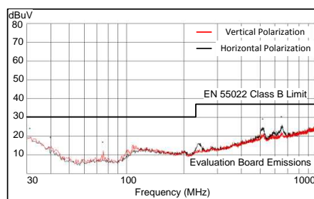
Radiated Emission Graph with V_{IN} = 12 V, V_{OUT} = 3.3 V, F_{SW} = 500 kHz, I_{OUT} = 0.5 A
