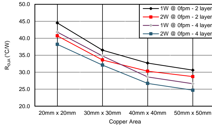
Figure 107. Measured R θJA vs PCB Copper Area on a 2-layer Board and a 4-layer Board
