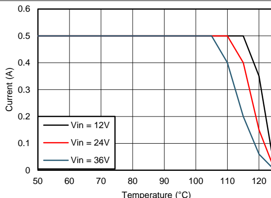
Figure 90. Derating Curve with R_{\theta JA} = 20^\circ\text{C/W}
