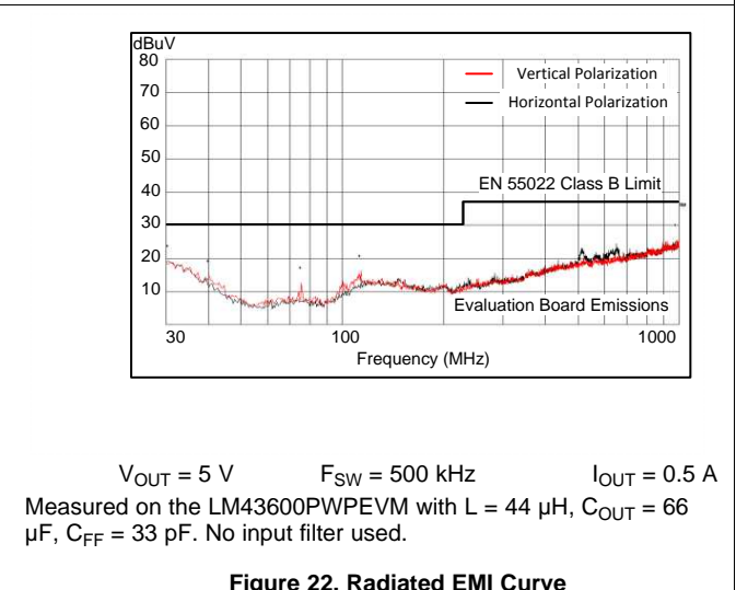
Figure 22. Radiated EMI Curve
