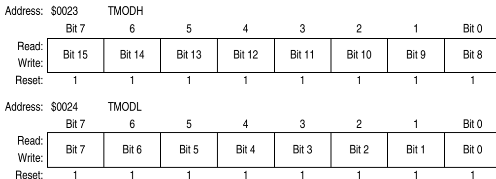
Figure 14-6. TIM Counter Modulo Registers (TMODH:TMODL)
