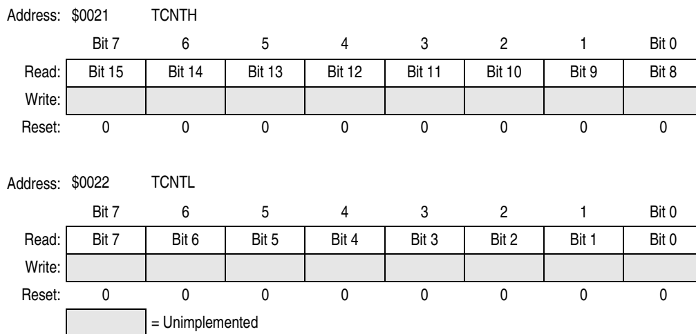
Figure 14-5. TIM Counter Registers (TCNTH:TCNTL)
