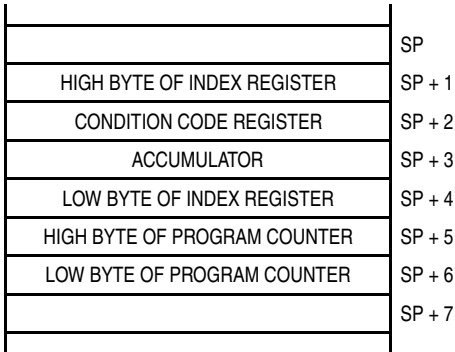
Figure 15-17. Stack Pointer at Monitor Mode Entry
