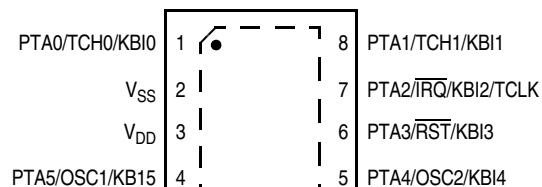
8-PIN ASSIGNMENT MC68HC908QT1 DFN
