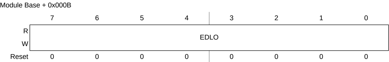
Figure 4-16. EEPROM Data Low Register (EDATALO)
