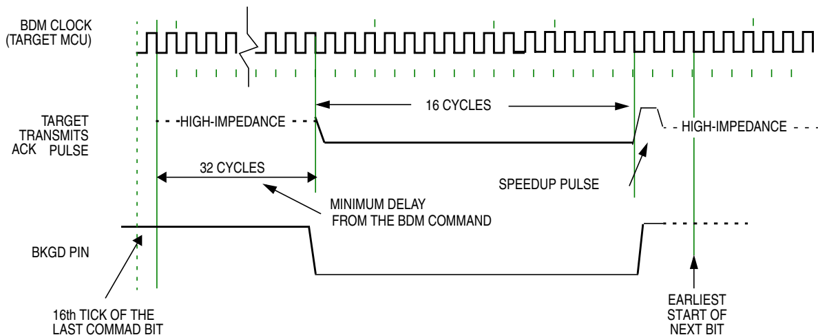
Figure 16-10. Target Acknowledge Pulse (ACK)
