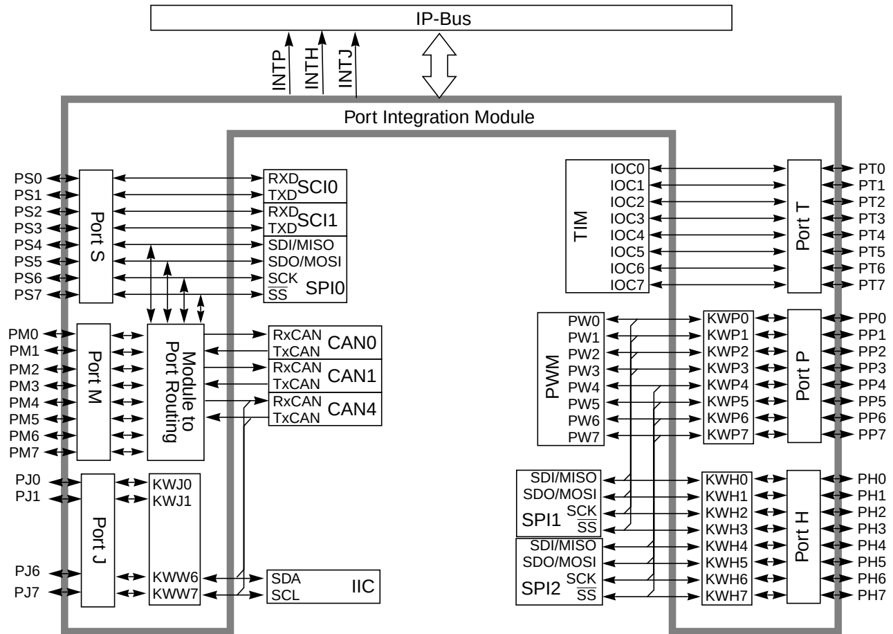
Figure 5-1. PIM9KT256 Block Diagram
