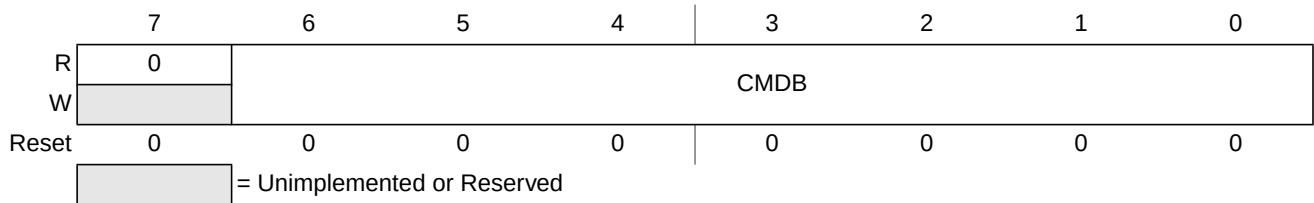
Figure 3-11. Flash Command Register (FCMD - NVM User Mode)
