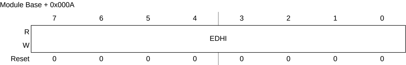
Figure 4-15. EEPROM Data High Register (EDATAHI)
