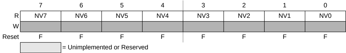
Figure 3-12. Flash Control Register (FCTL)
