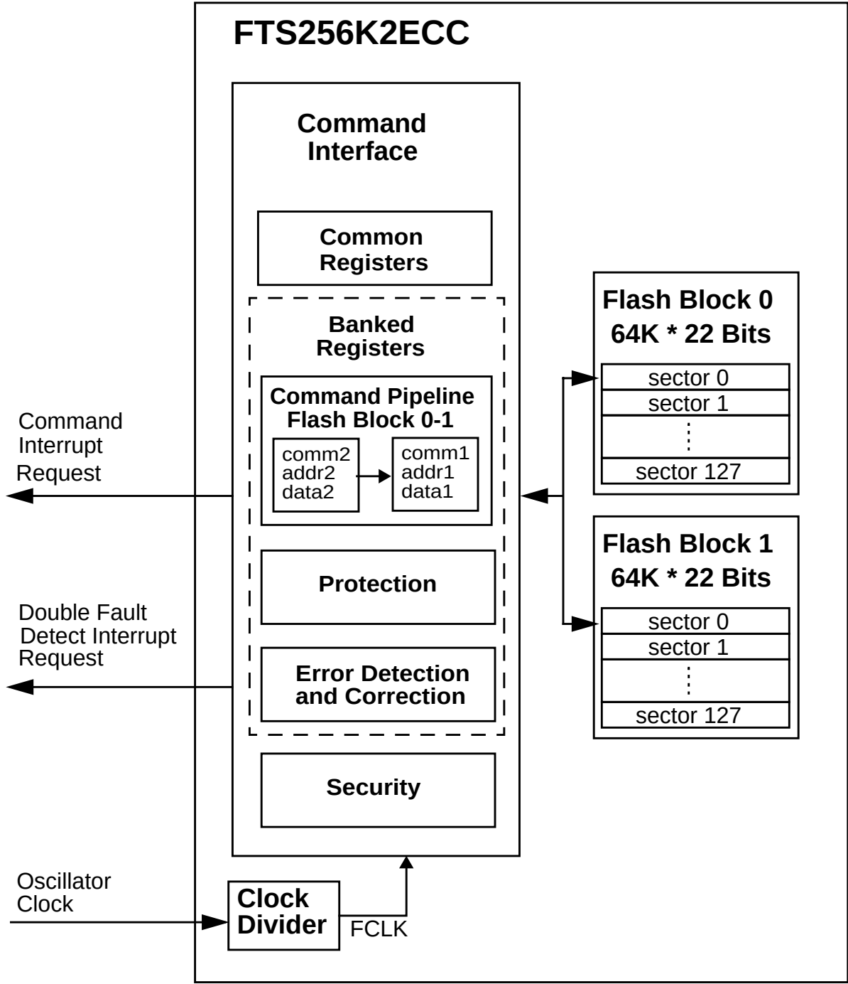
Figure 2-1. FTS256K2ECC Block Diagram
