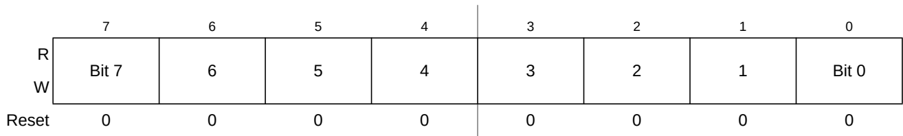
Figure 19-5. Data Direction Register B (DDRB)
