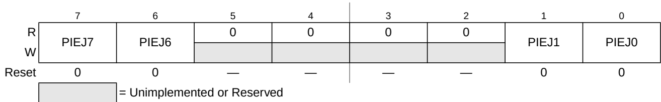
Figure 5-45. Port J Interrupt Enable Register (PIEJ)
