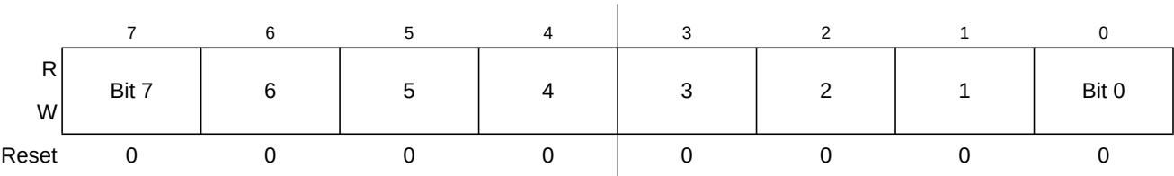
Figure 19-4. Data Direction Register A (DDRA)
