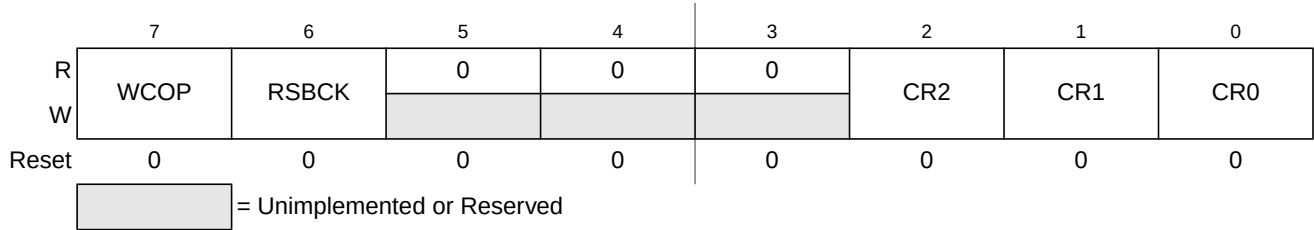
Figure 6-12. CRG COP Control Register (COPCTL)
