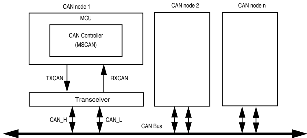
Figure 10-2. CAN System
