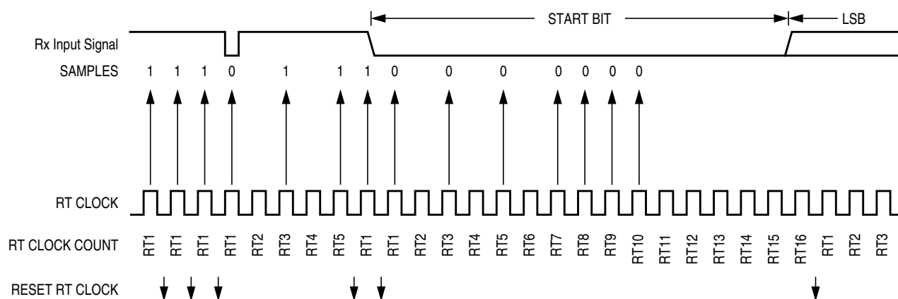
Figure 11-14. Start Bit Search Example 1
