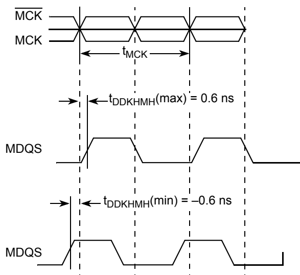
Figure 5. Timing Diagram for t_{DDKMH}
