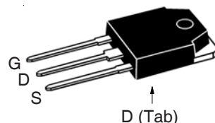
TO-264 (IXTK)
