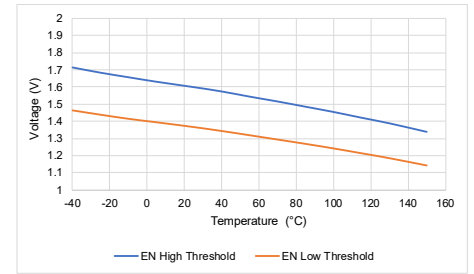
EN High and Low Thresholds vs. Temperature
