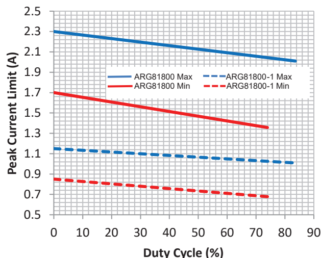
Figure 3: Peak Current Limit vs. Duty Cycle
