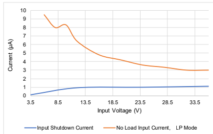
Input Current vs. Input Voltage
