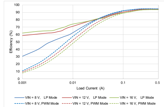
Efficiency vs. Load Current V_{OUT} = 5.0\text{ V} , f_{SW} = 400\text{ kHz}
