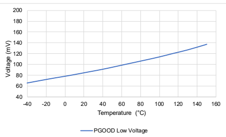
PGOOD Low Voltage vs. Temperature
