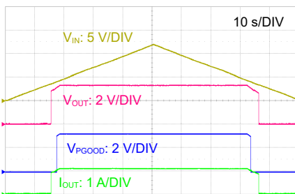
V_{IN} Slow Ramp Up and Ramp Down V_{OUT} = 3.3\text{ V} , I_{OUT} = 1.0\text{ A} , PWM Mode
