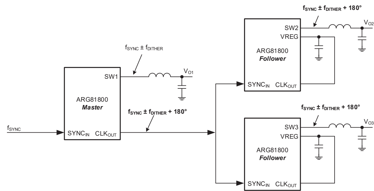
Figure 1: Master-Follower Configuration
