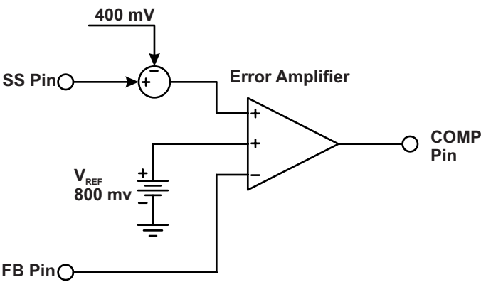
Figure 2: ARG81800 Error Amplifier
