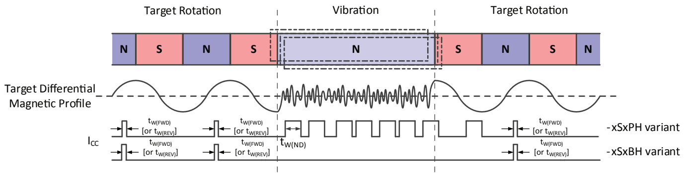
Figure 15: Vibration Behavior
