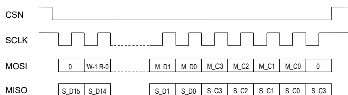
Figure 49: Twenty-One Bit SPI Transaction
