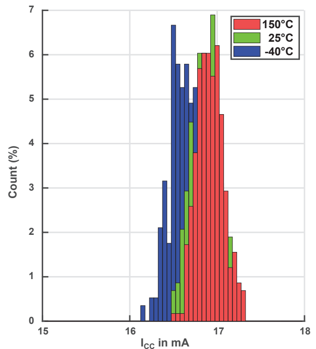
Figure 10: I_{CC} Distribution over Temperature ( V_{CC} = 16.0 V)
