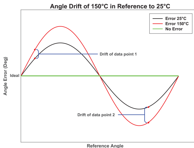
Figure 71: Angle Drift of 150°C in Reference to 25°C [1]
