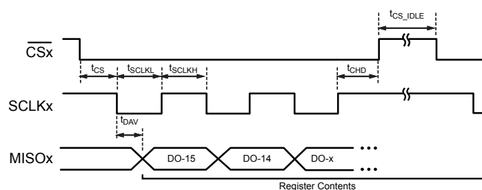
Figure 45: SPI Interface Timings Output
