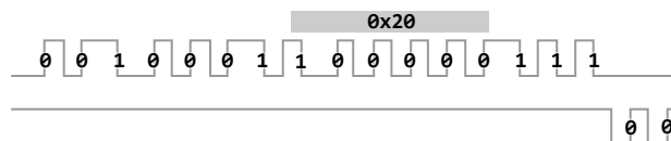
Figure 57: Target ID = [0 0 0 1], "angle" = 0x20, CRC = '111'
