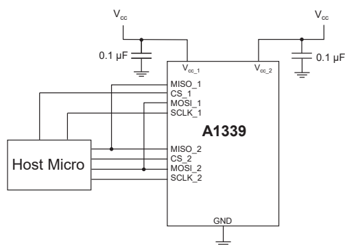
Figure 72: Separate SCLK Lines
