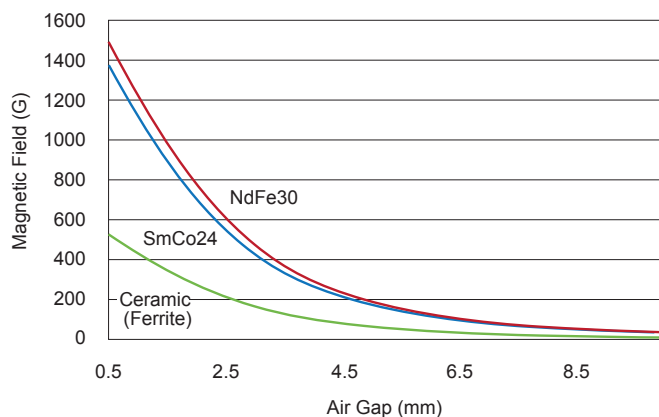
Figure 64: Magnetic Field versus Air Gap for a magnet 6 mm in diameter and 2.5 mm thick.
