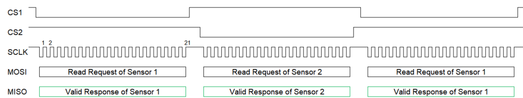
Figure 77: SPI Implementation using 21-bit packets; data contents are valid; no false IER flag generation
