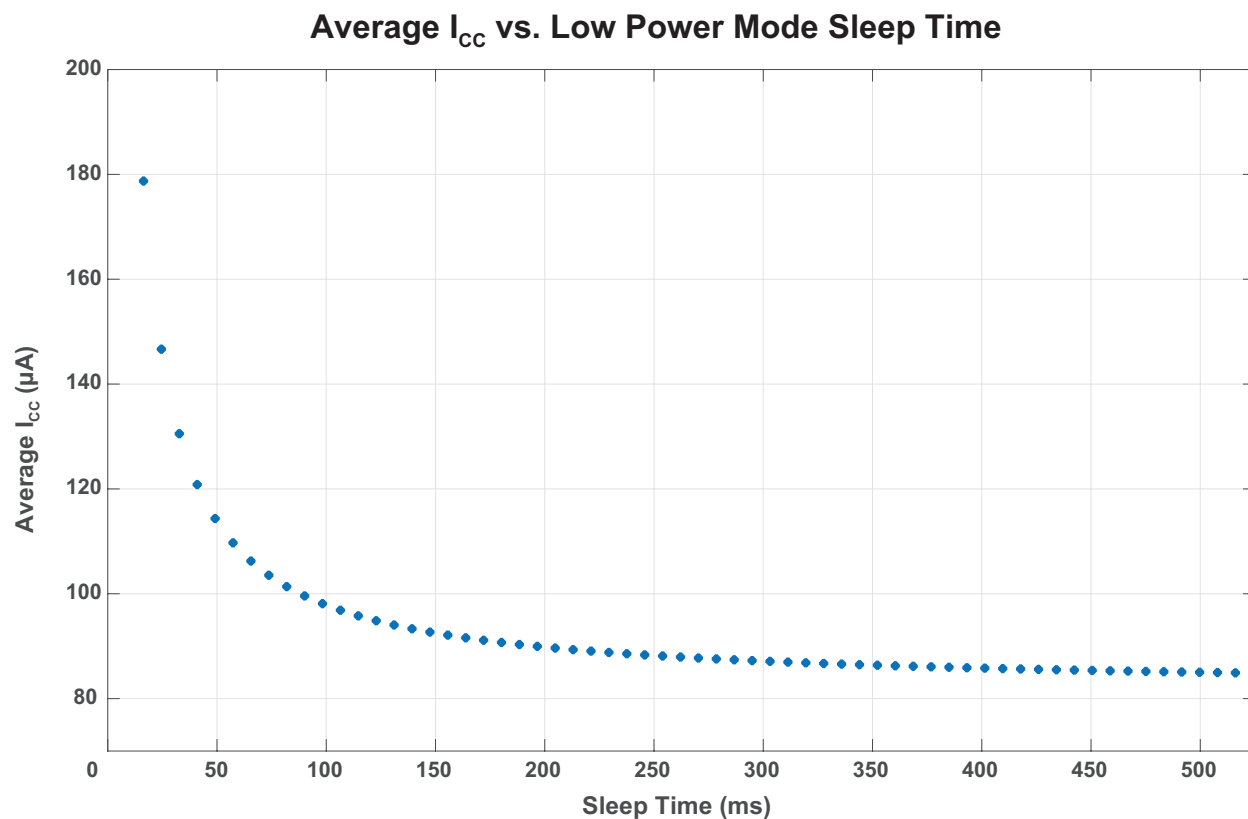
Figure 35: Typical Average Low Power Mode Current Consumption; T_A = 25^\circ C , V_{CC} = 16 V
