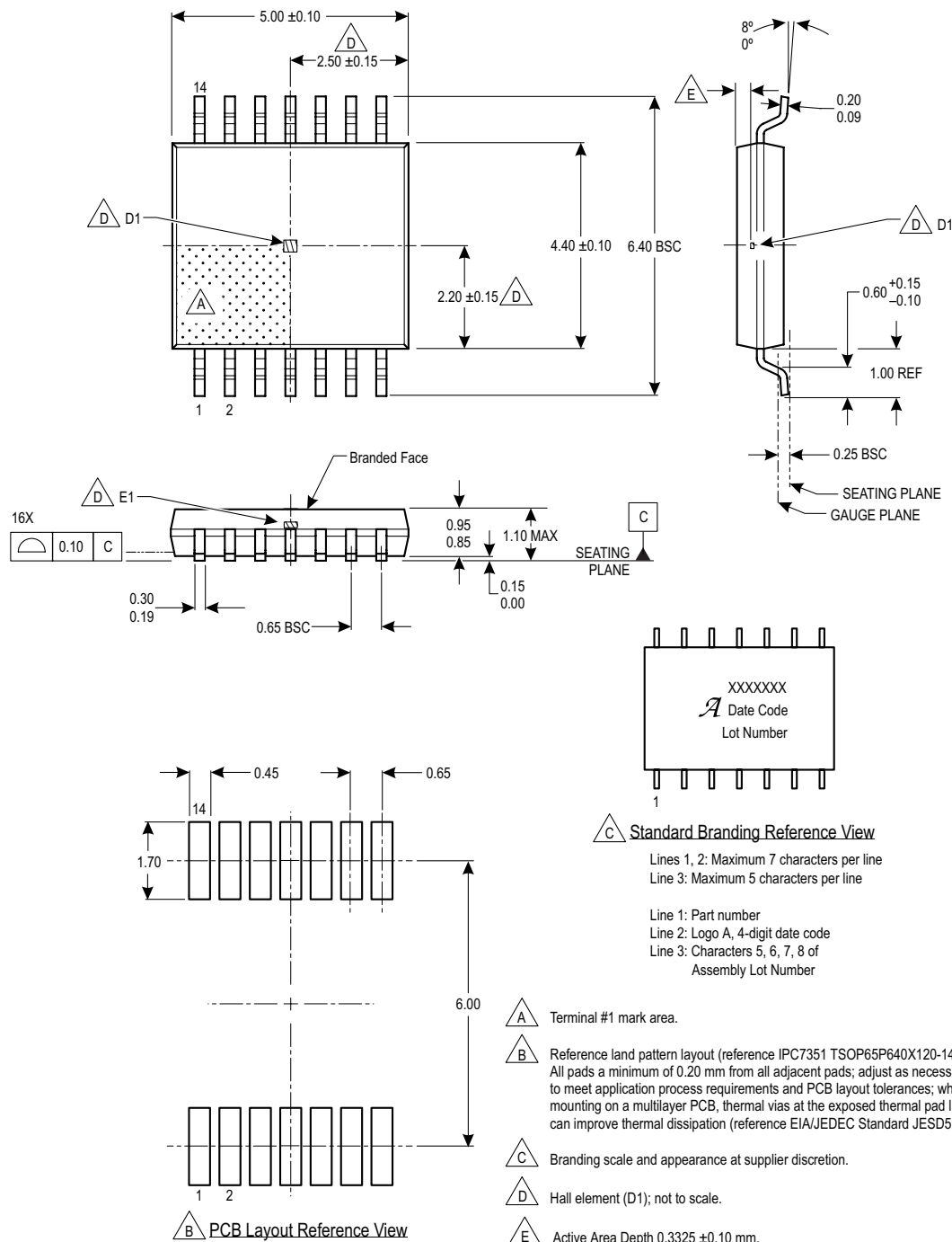
Figure 69: Package LE, 14-Pin TSSOP
