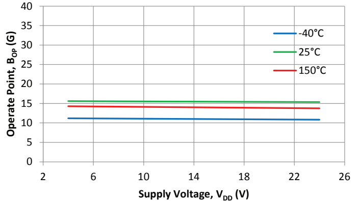
Avg. OUTPUTB Operate Point vs. Supply Voltage
