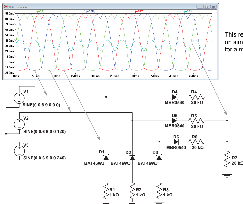
Figure 40: SPICE Simulation Example for Filtered BEMF Signal
