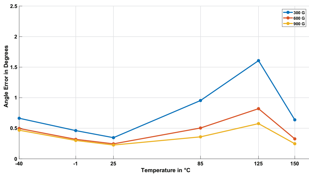
Figure 11: Average Angle Error over Temperature Across 10 Devices. Recommended operating range: 300 G and above.
