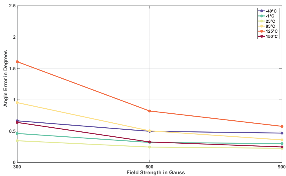
Figure 12: Average Angle Error over Field. Recommended operating range: 300 G and above.
