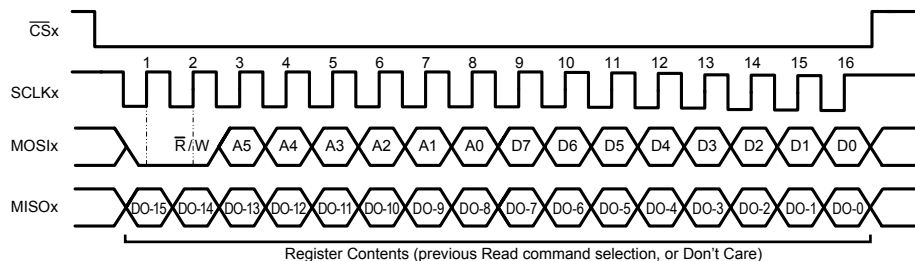
Figure 50: SPI Read and Write Pulse Sequences
