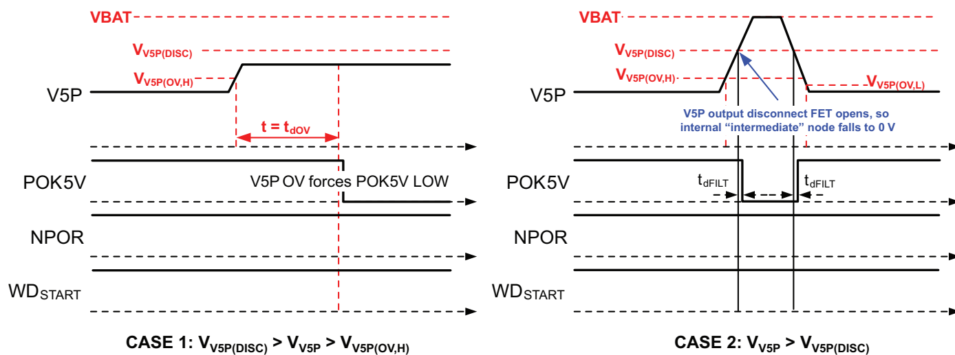
Figure 15: Overtoltage Cases for V5P
