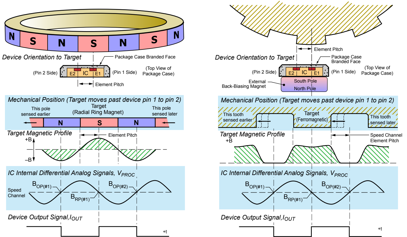
Figure 5: Basic Operation
