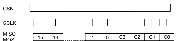
Figure 37: Seventeen Bit SPI Transaction
