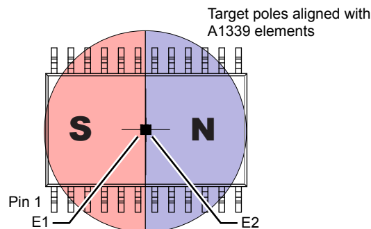
Figure 50: Orientation of Magnet Relative to Primary and Secondary Die
