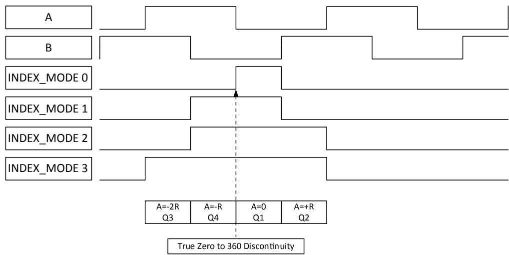
Figure 19: Index Pulse
