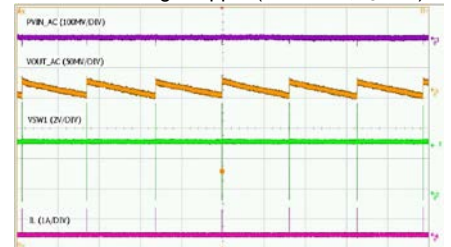
Time-1ms/div
