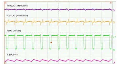
Time-500ns/div
