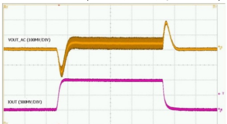
Time-100μs/div
