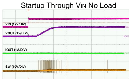
Time-500 \mu\text{s/div}
