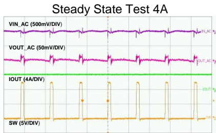
Time-1 \mu\text{s/div}
