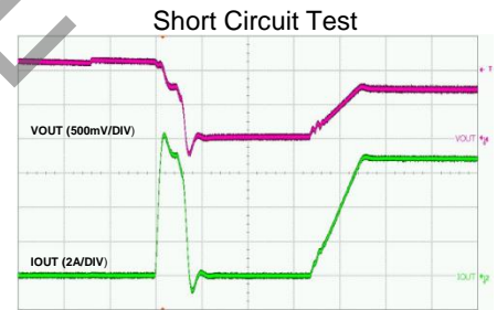
Time-100 \mu\text{s/div}
