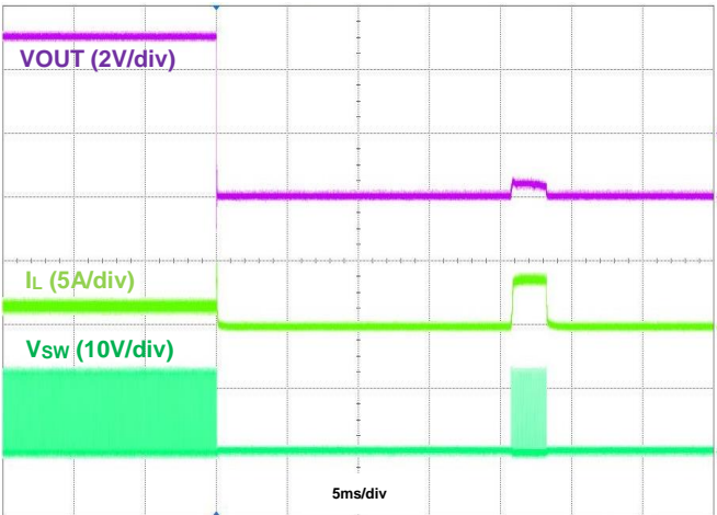
Figure 22. Output Short Protection, I_{OUT} = 1.5\text{A}
