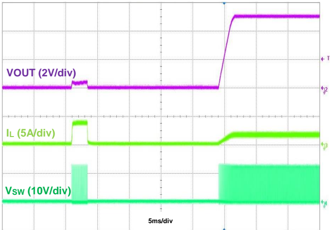
Figure 23. Output Short Recovery, I_{OUT} = 1.5\text{A}
