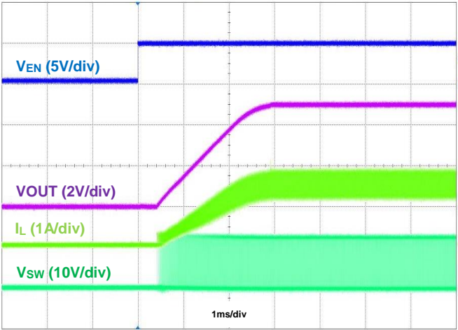
Figure 20. Startup Using EN, I_{OUT} = 1.5\text{A}
