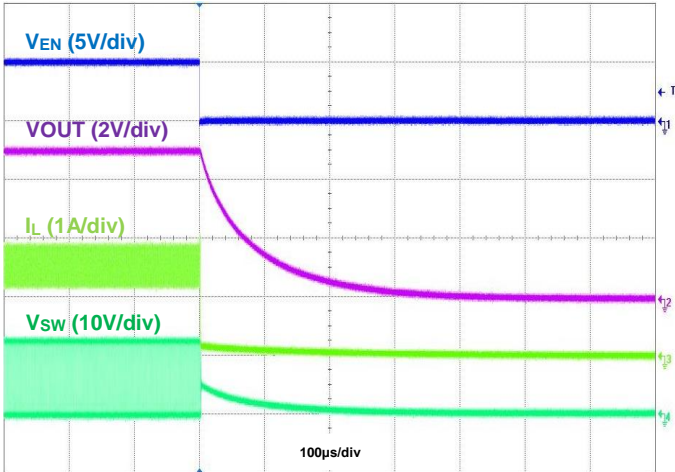
Figure 21. Shutdown Using EN, I_{OUT} = 1.5\text{A}
