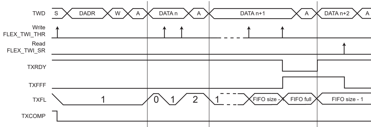
Figure 39-136. RXRDY Behavior when RXRDYM = 0 in Master and Slave Modes
