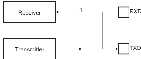
Figure 39-69. Remote Loopback Mode Configuration
