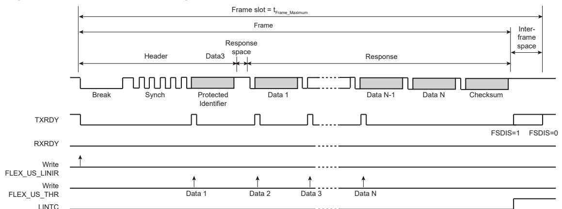
Figure 39-45. Master Node Configuration, NACT = PUBLISH
