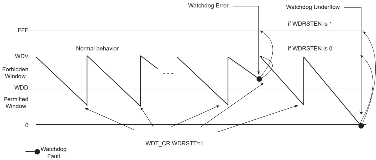
Figure 21-2. Watchdog Behavior
