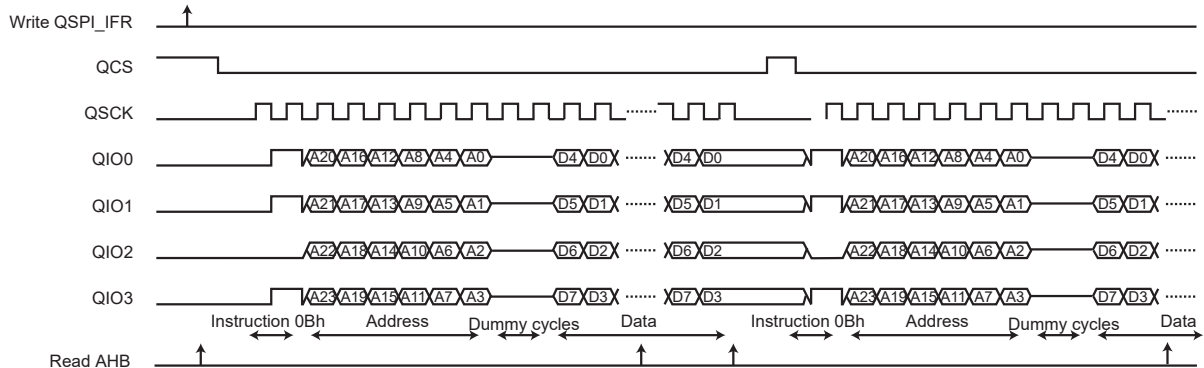
Figure 38-18. Instruction Transmission Waveform 8
