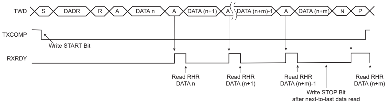
Figure 39-98. Master Read Clock Stretching with Multiple Data Bytes
