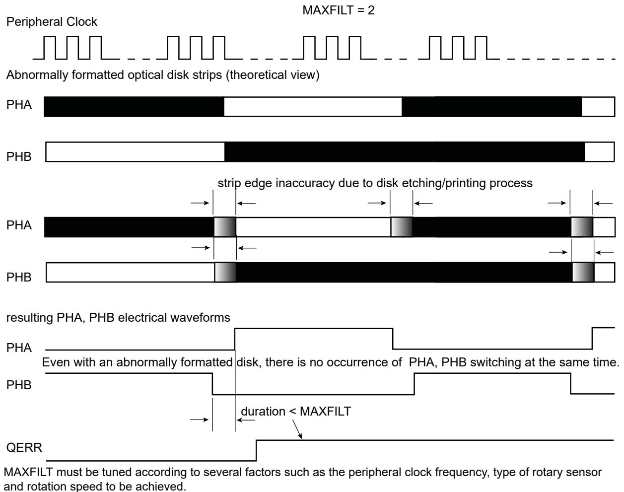
Figure 41-21. Quadrature Error Detection
