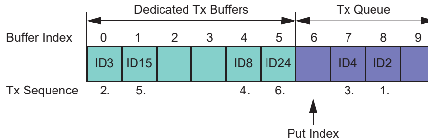
Figure 40-11. Example of Mixed Configuration Dedicated Tx Buffers / Tx Queue
