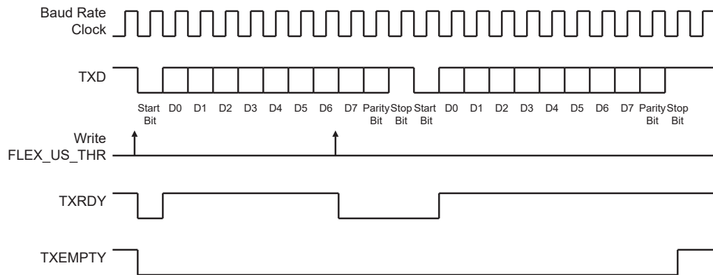
Figure 39-6. Transmitter Status
