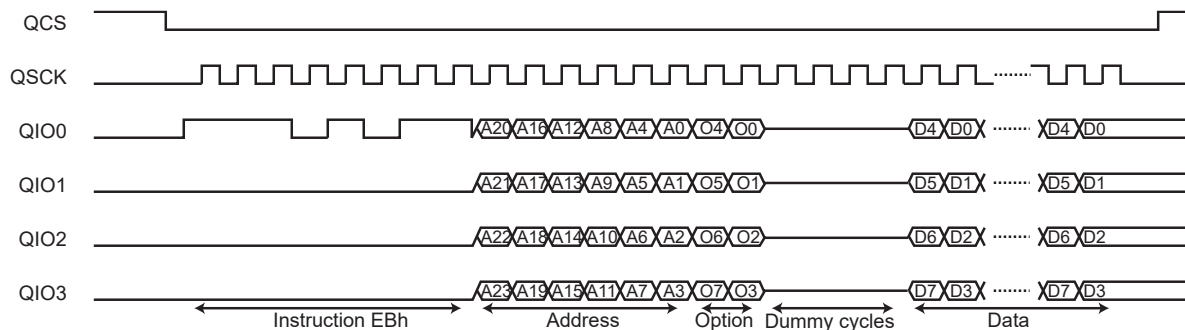
Figure 38-8. Instruction Frame
