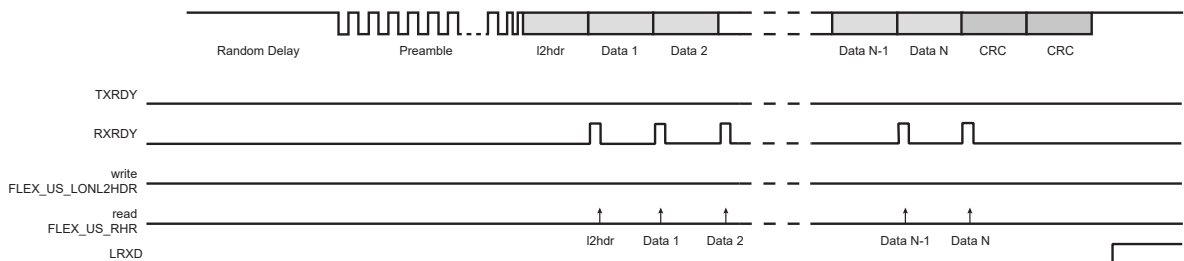
Figure 39-62. Rx Frame
