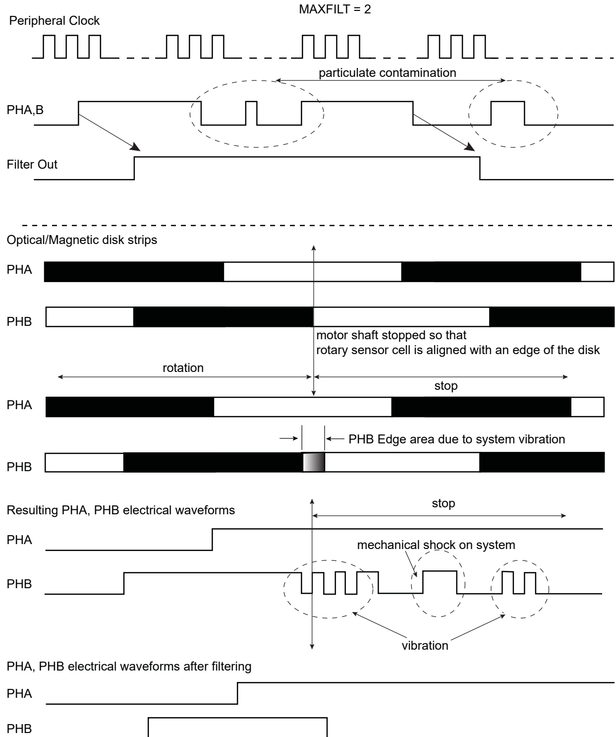
Figure 41-19. Filtering Examples
