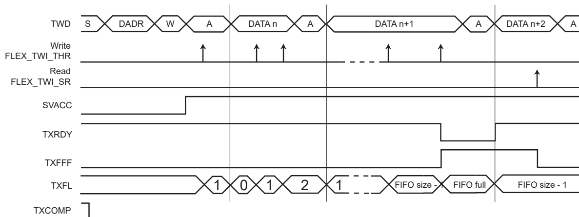
Figure 39-137. TXRDY Behavior when TXRDYM = 0 in Slave Mode
