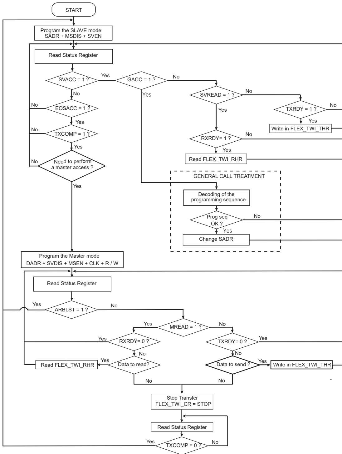
Figure 39-119. Multi-Master Mode
