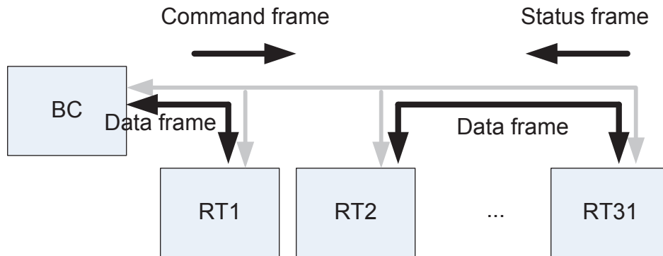
Figure 35-3. 1553 Frames
