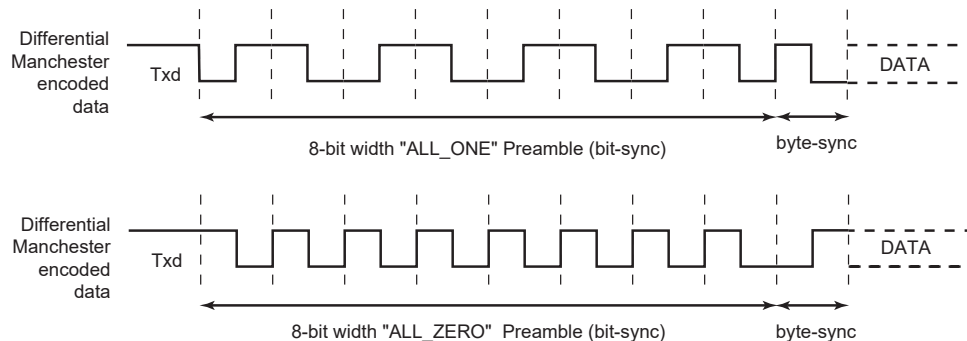
Figure 39-57. Preamble Patterns
