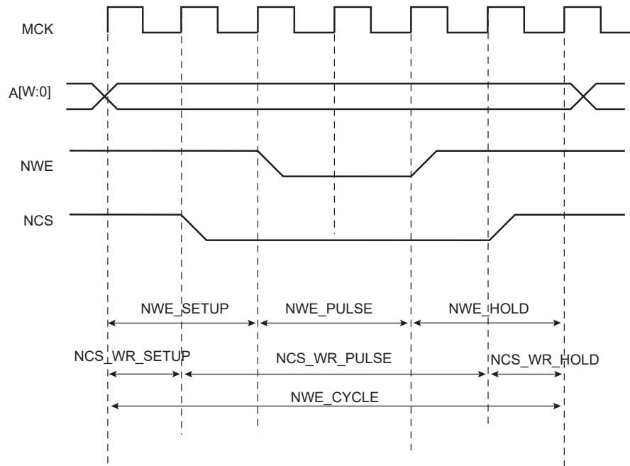
Figure 31-5. Write Cycle
