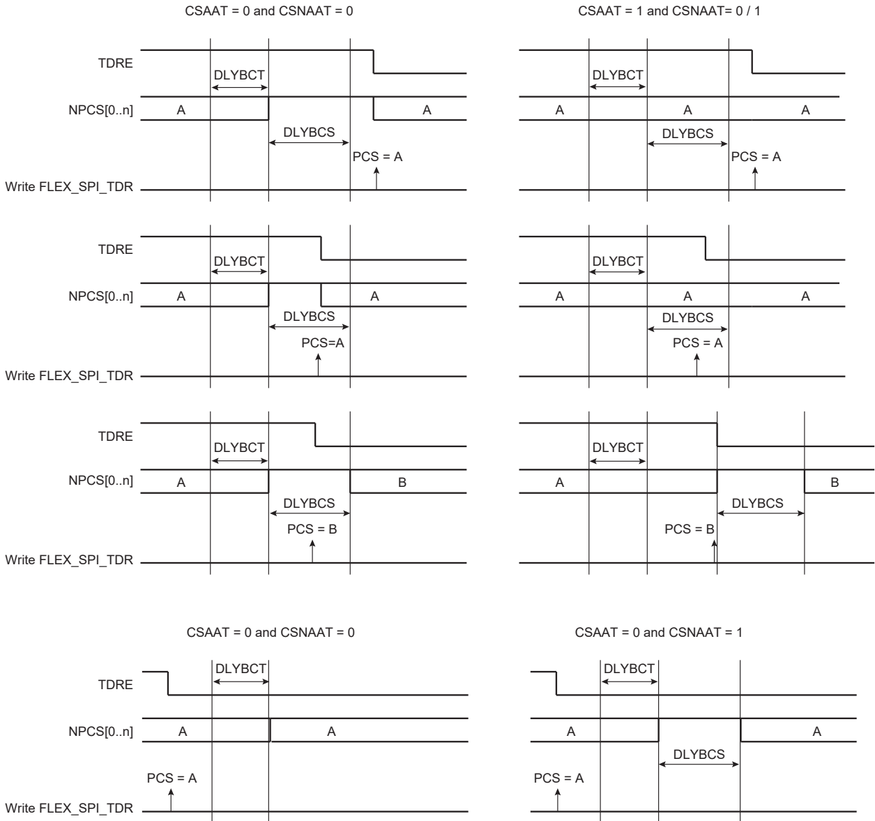
Figure 39-83. Peripheral Deselection
