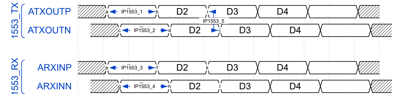
Figure 47-7. 1553 Characteristics
