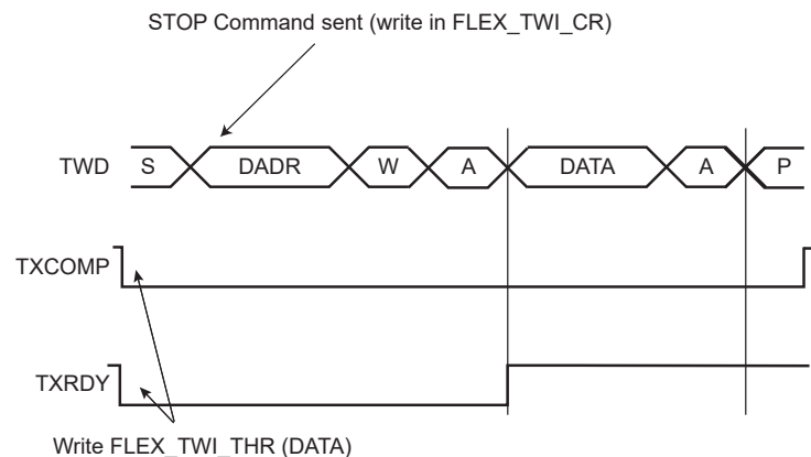
Figure 39-93. Master Write with One Data Byte
