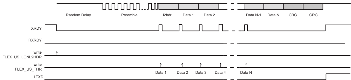
Figure 39-61. Tx Frame
