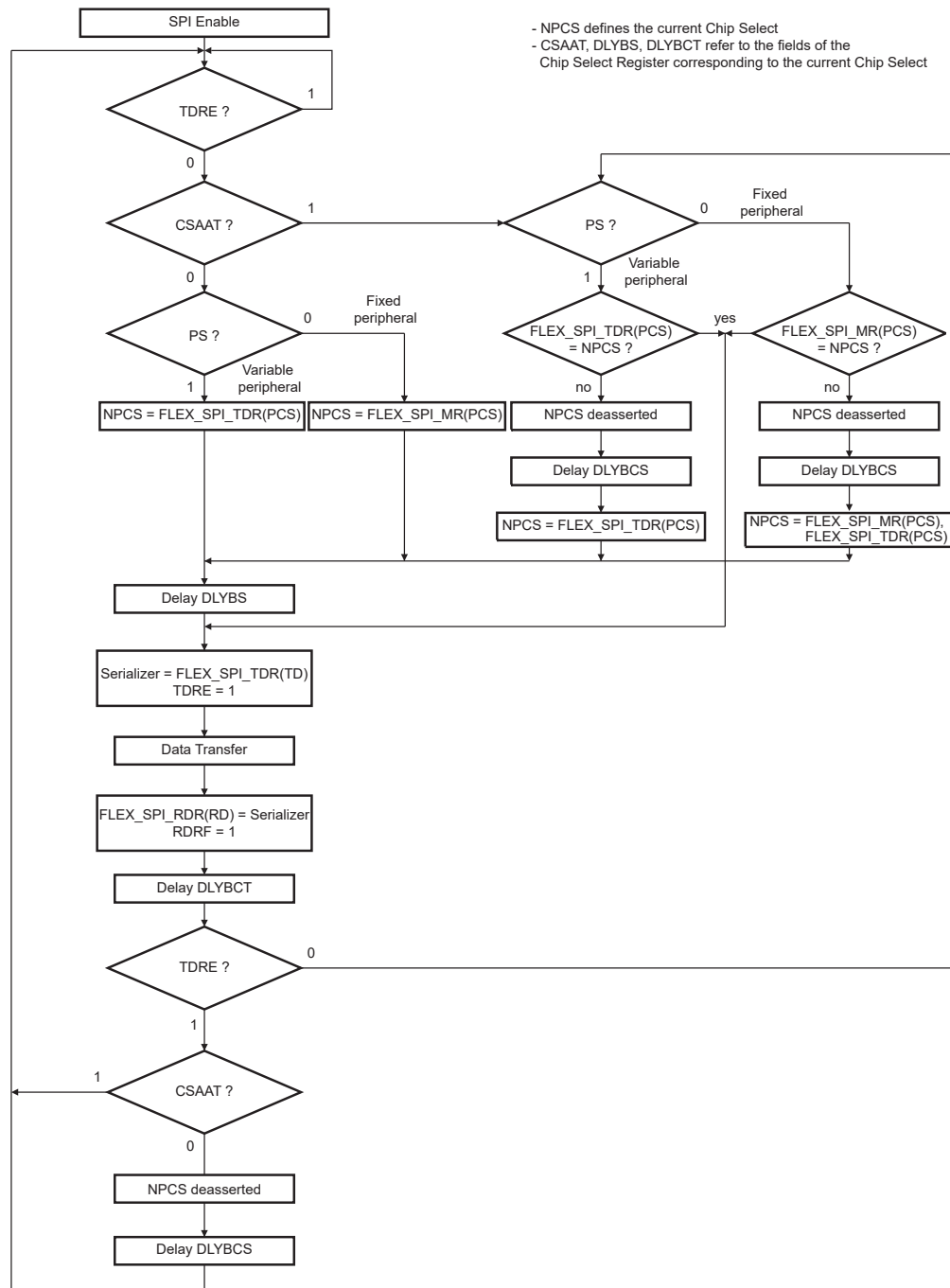
Figure 39-79. Master Mode
