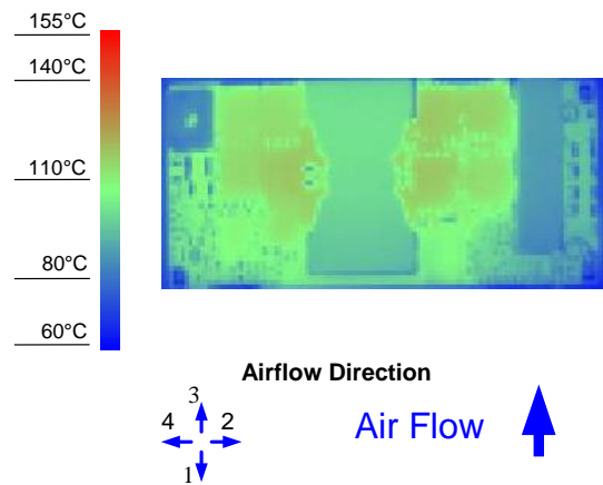
Figure 10. Thermal Image for Airflow Direction 3 (20A output, 55°C ambient, 200 LFM, typical Vin, open frame unit, solder interface)
