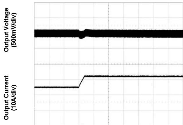
Figure 6. Transient Load Response (typical Vin, load current steps from 50% to 75% at a slow rate 0.1A/µs, 1,000µF external output capacitance)
