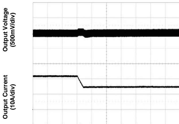
Figure 5. Transient Load Response (typical Vin, load current steps from 75% to 50% at a slow rate 0.1A/µs, 1,000µF external output capacitance)
