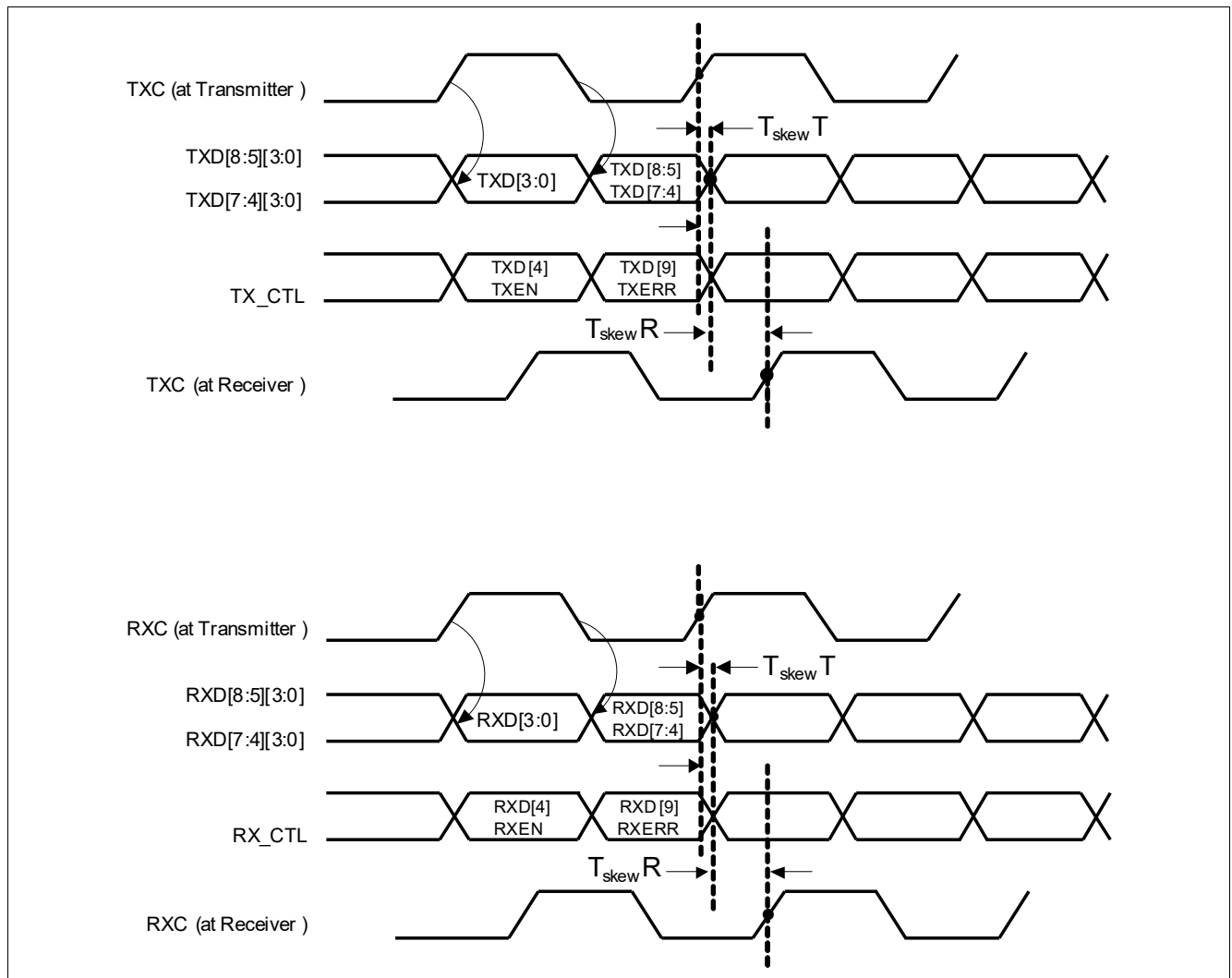
Figure 53 Timing Diagram of the RGMII
