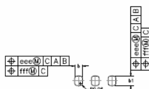
DETAIL "B" (2:1)(101X)
