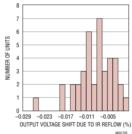
Figure 21. Output Voltage Shift Due to IR Reflow
